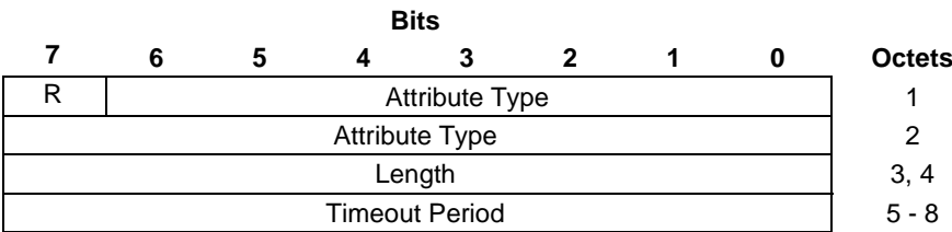
Figure 8.2.4.2-1: TIMEOUT_PERIOD_FOR_LIVENESS_CHECK attribute
