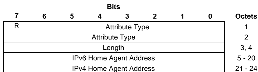
Figure 8.2.4.1-1: HOME_AGENT_ADDRESS attribute
