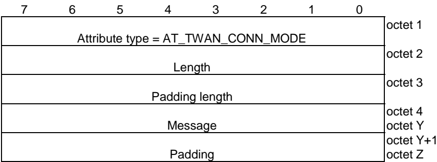
Figure 8.2.7.1-1: AT_TWAN_CONN_MODE attribute
