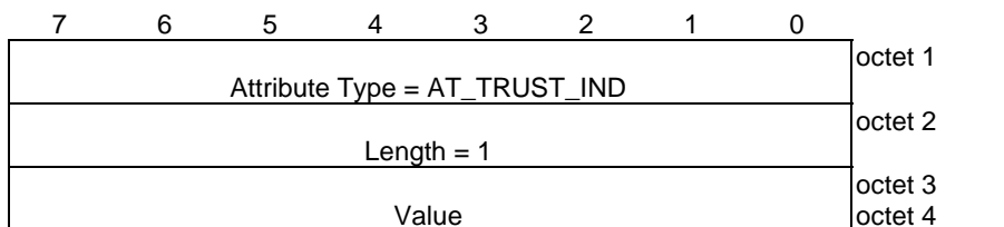
Figure 8.2.3.1-1: AT_TRUST_IND attribute
