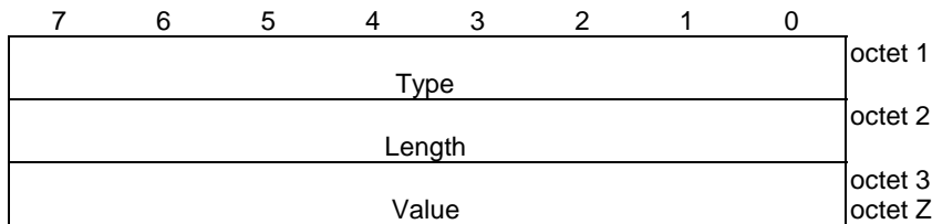
Figure 8.1.4.2-1: Item
