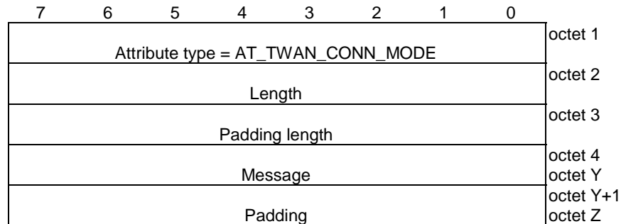
Figure 8.2.7.1-1: AT_TWAN_CONN_MODE attribute
