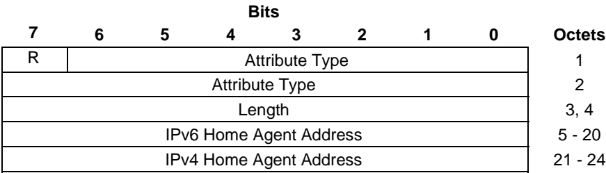
Figure 8.2.4.1-1: HOME_AGENT_ADDRESS attribute
