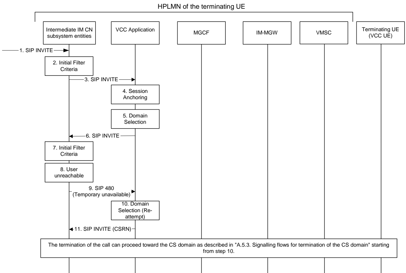
Figure A.5.6-1: Call termination delivery attempt failure to the IM CN subsystem
