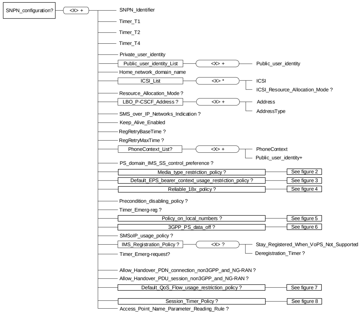
Figure 9: SNPN configuration
