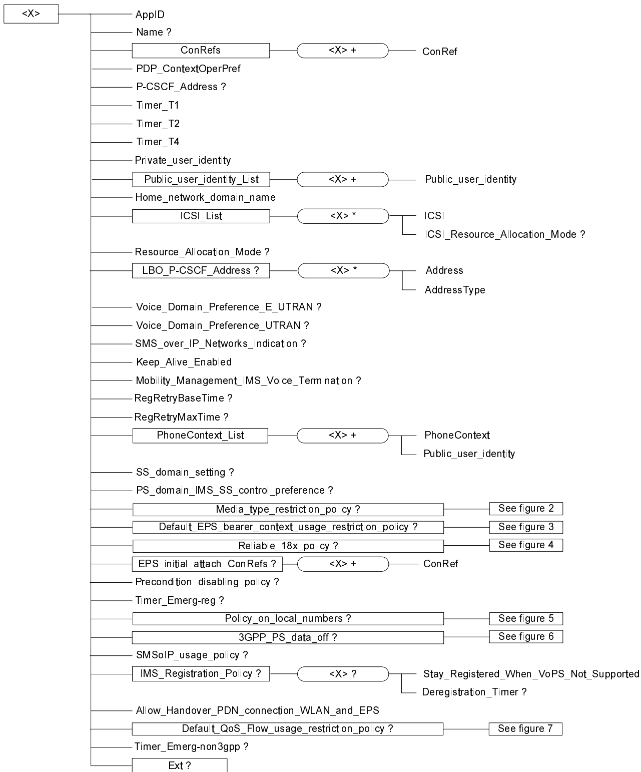
Figure 1: The 3GPP IMS Management Object
