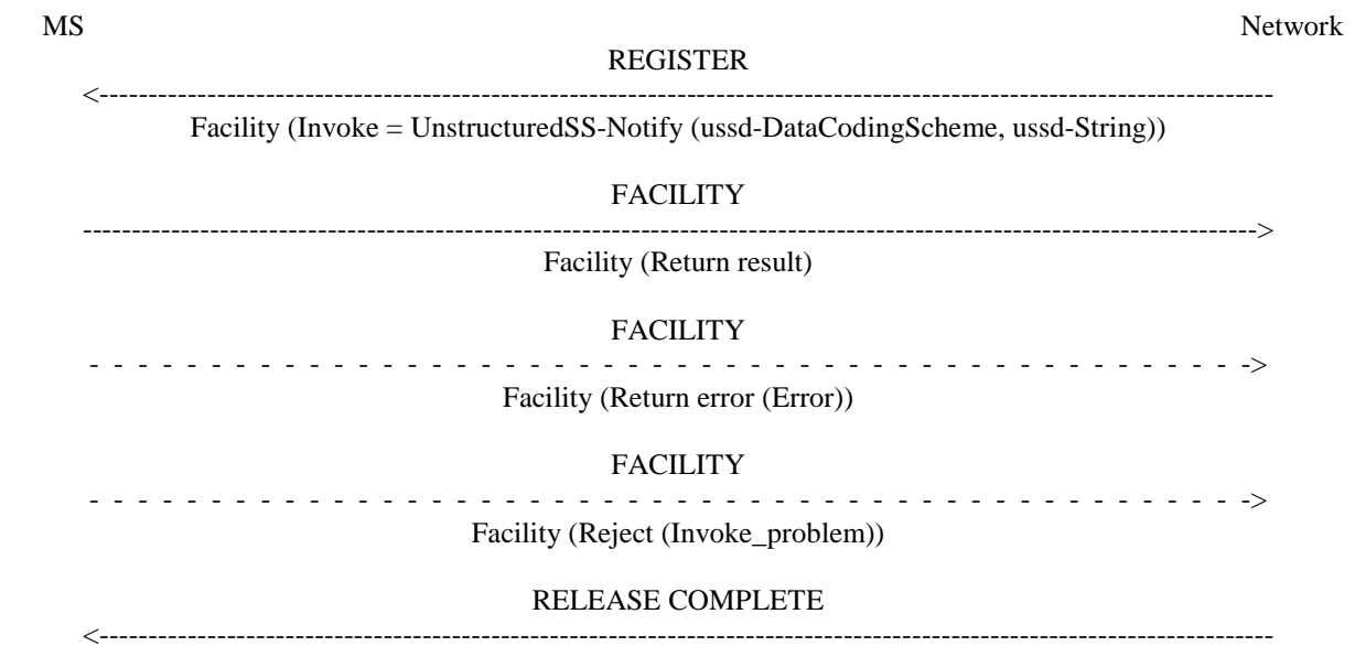
Figure 5.3: Single network initiated USSD notification
