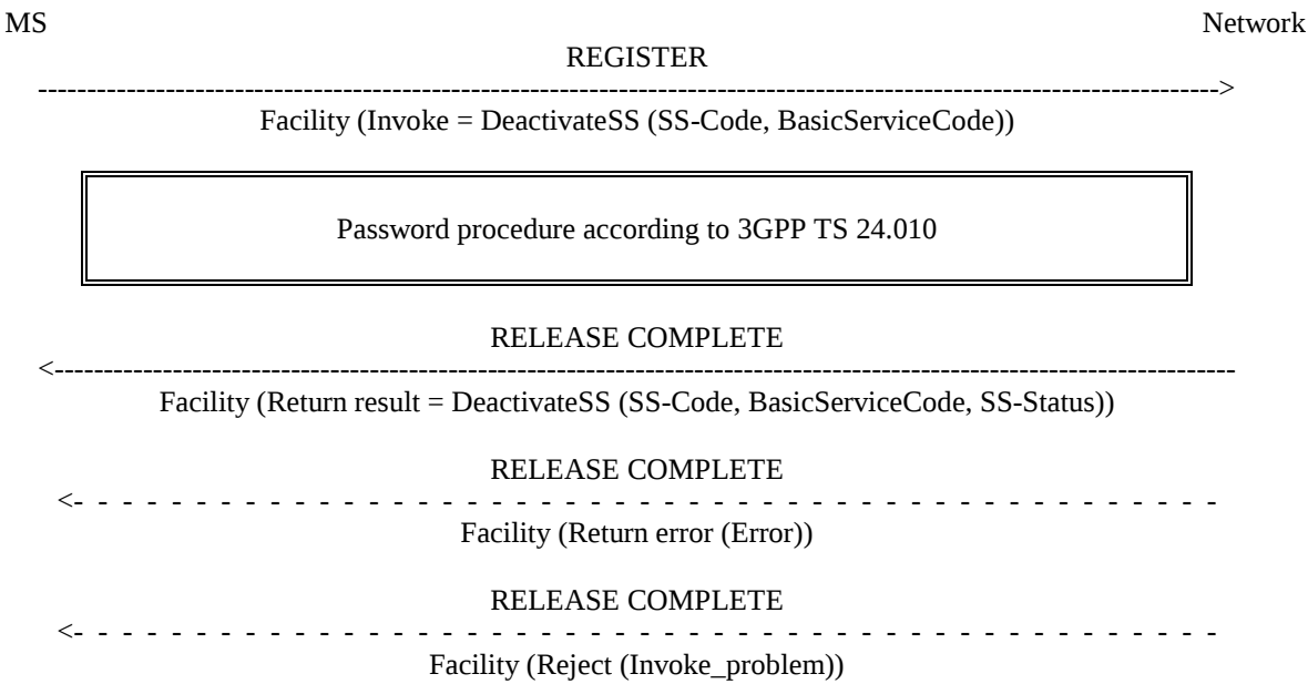
Figure 1.3: Deactivation of barring of outgoing calls
