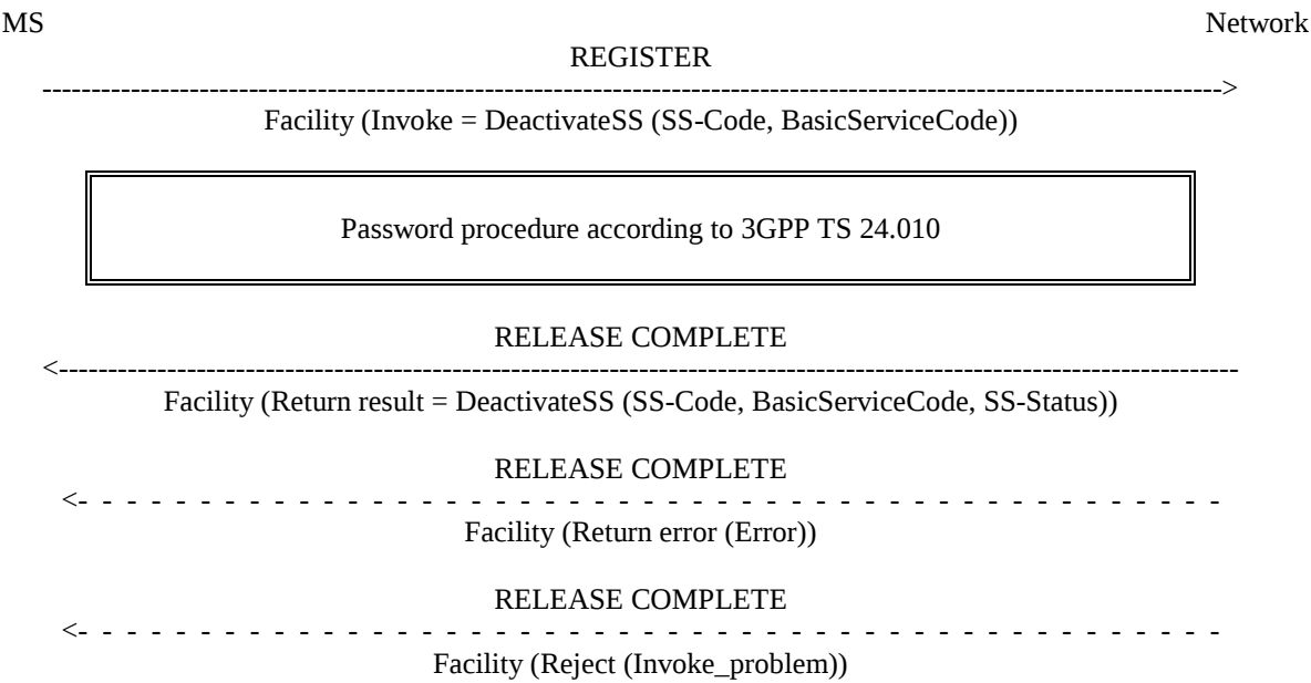
Figure 2.3: Deactivation of barring of incoming calls
