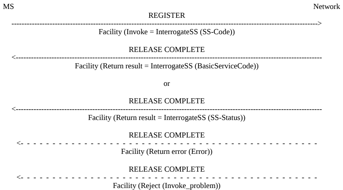
Figure 1.4: Interrogation of a barring program
