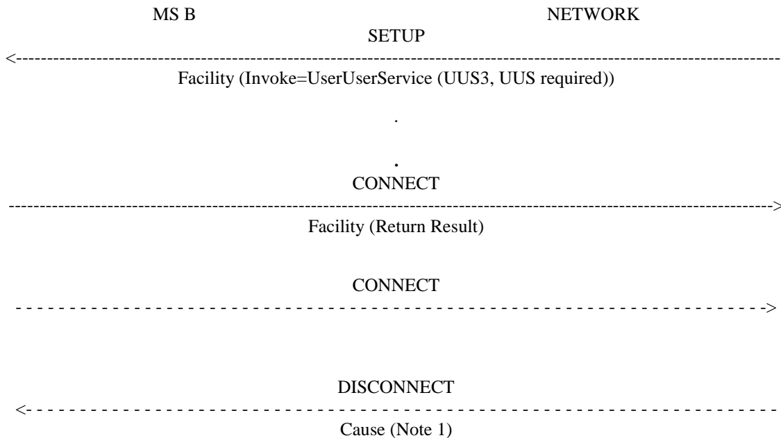
Figure 16: Request for explicit activation of UUS3 when originating a call, UUS required
