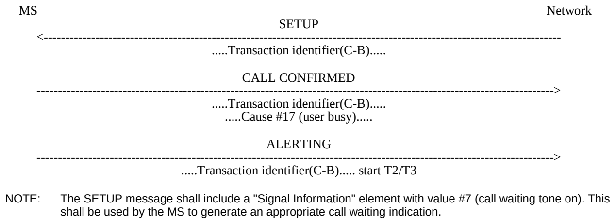
Figure 1.1: Call indication to the mobile station on arrival of an incoming call and call confirmation from the mobile station
