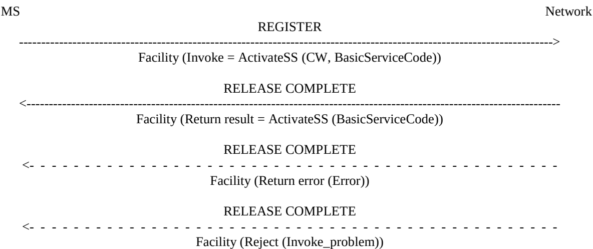
Figure 1.4: Activation of call waiting
