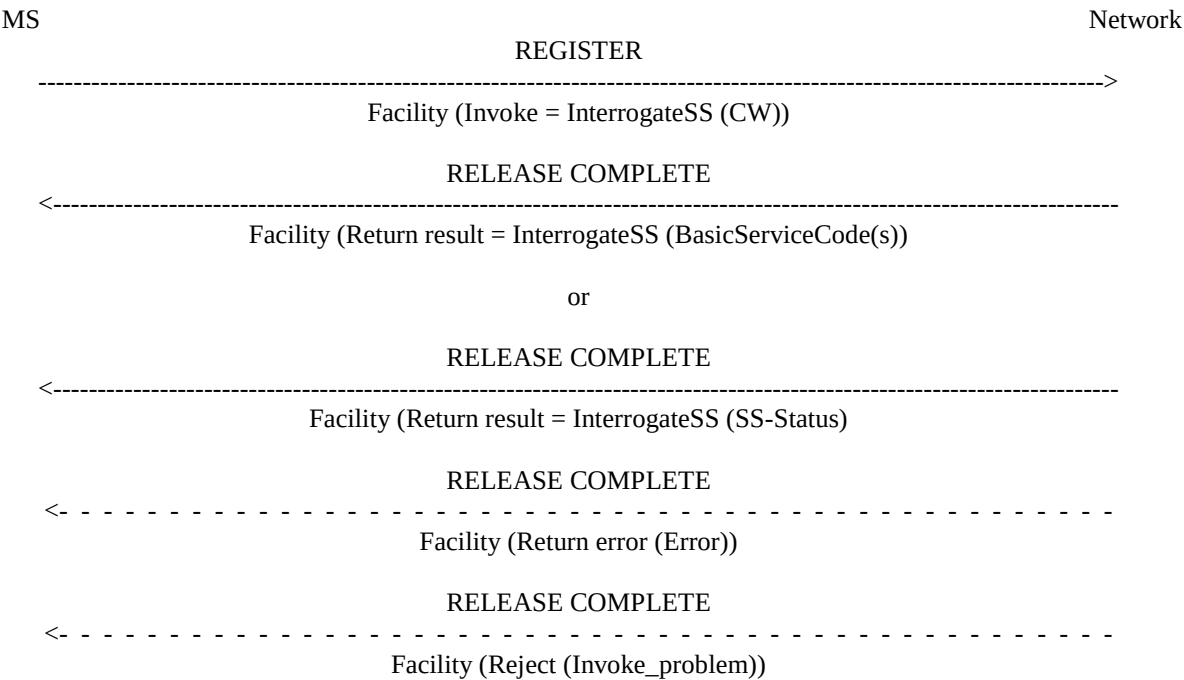
Figure 1.6: Interrogation of call waiting
