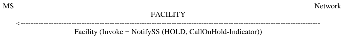
Figure 2.4: Notification to the held mobile party that the held call has been retrieved
