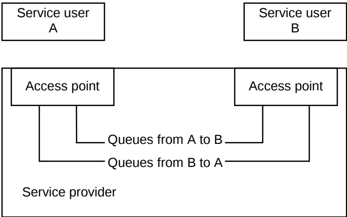
Figure 7: Queue Model
