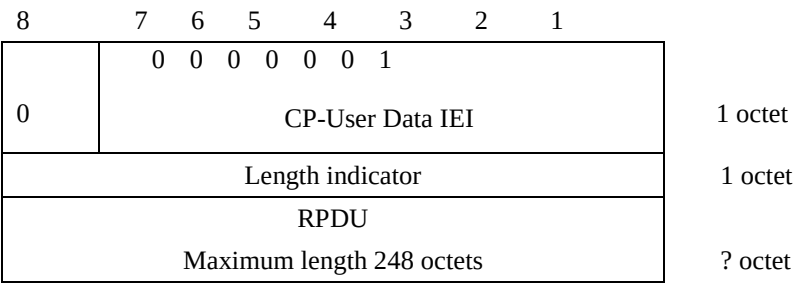
Figure 8.2/3GPP TS 24.011: CP-User data element layout
