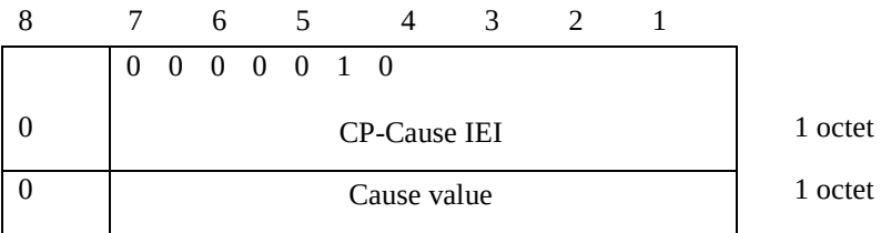
Figure 8.3/3GPP TS 24.011: CP-Cause element layout
