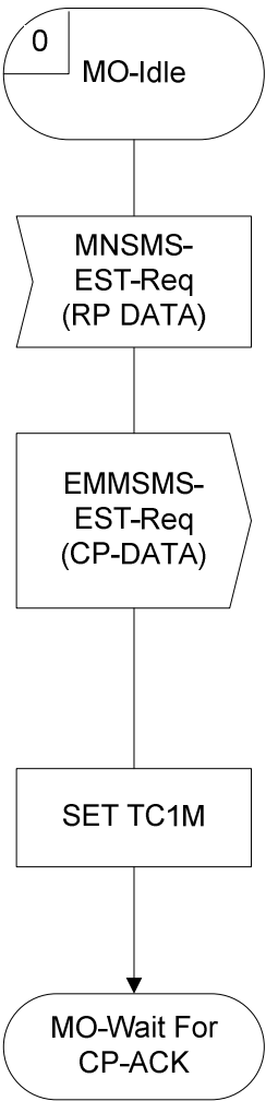
MO-SMC-EP entity on MS-side for EPS when the UE is using EPS services with control plane Clot EPS optimization SDL-31a
