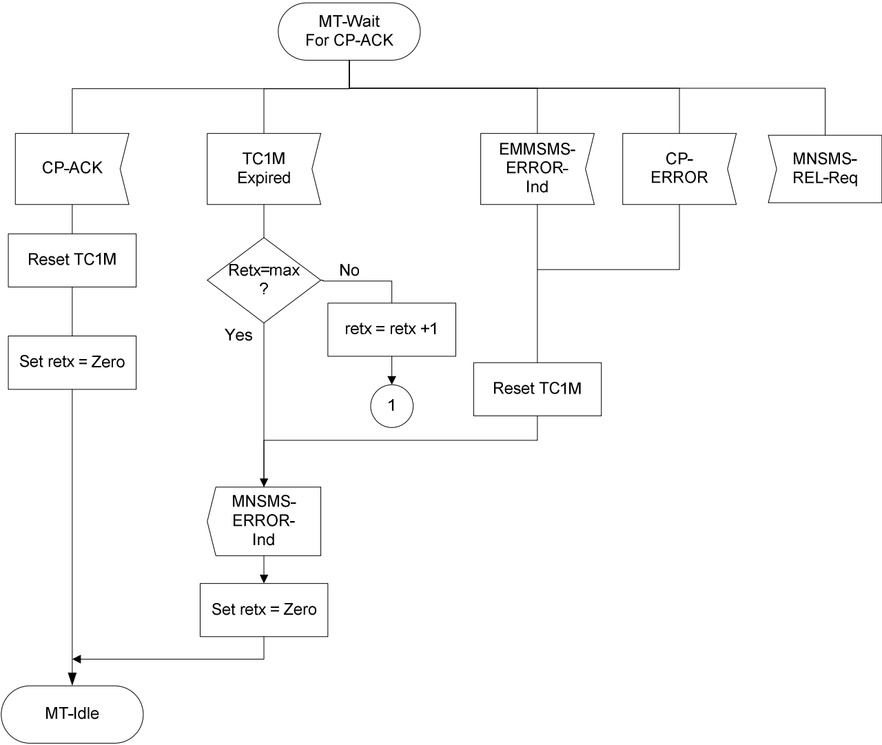
MT-SMC-EP entity on MS-side for EPS SDL-36
