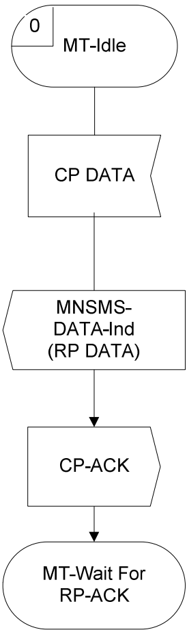
MT-SMC-5G entity on MS-side for 5GS SDL-46
