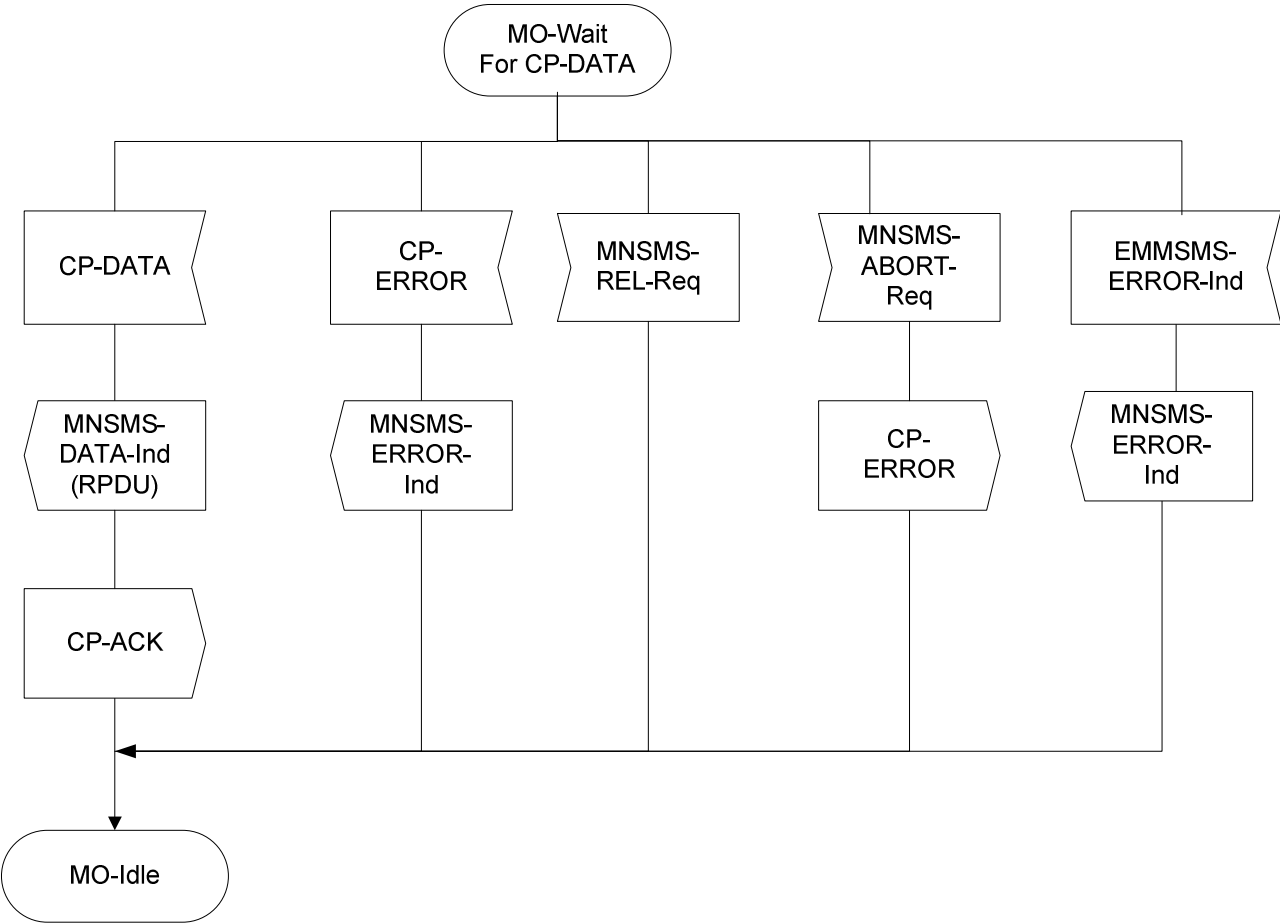
MO-SMC-EP entity on MS-side for EPS SDL-33
