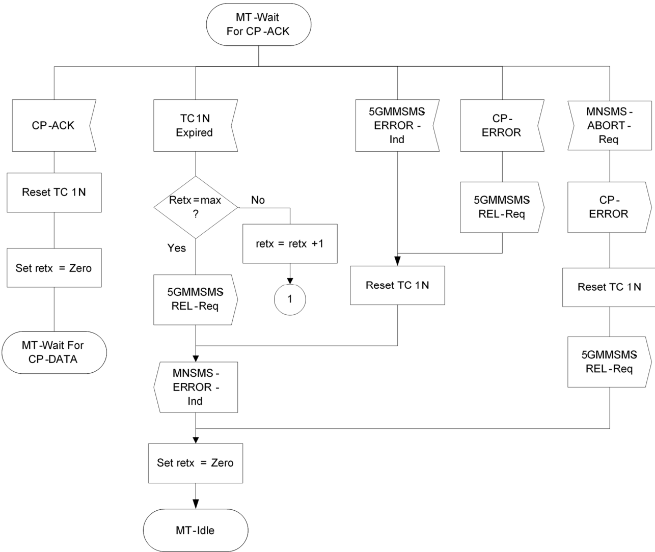
MT-SMC-5G entity on Network-side for 5GS when packet-switched service is used SDL-41
