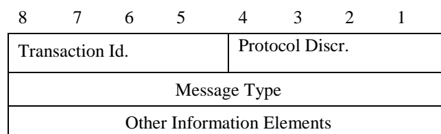
Figure 8.1/3GPP TS 24.011
