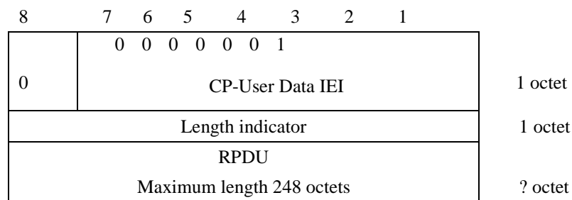
Figure 8.2/3GPP TS 24.011: CP-User data element layout
