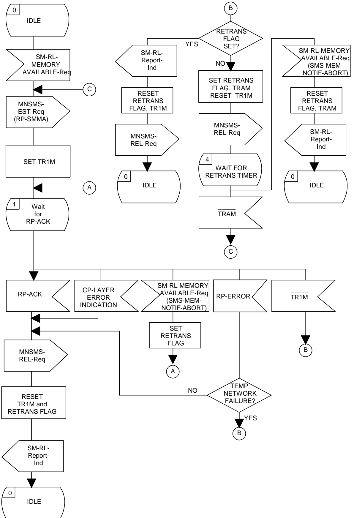
SMR-entity on MS-side Memory Available Notification SDL-3
