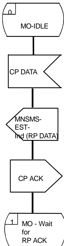
MO-SMC-GP entity on Network side for GPRS SDL-19
