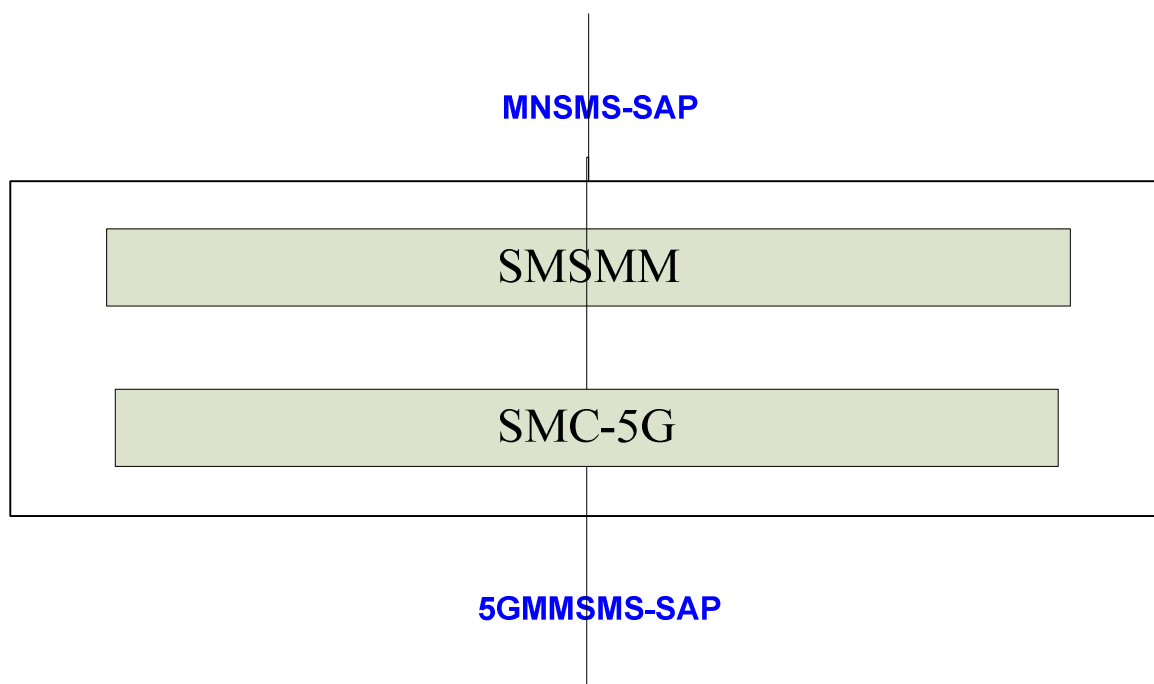
Figure 2.5B/3GPP TS 24.011: 5GSMS entity for MS in N1 mode
