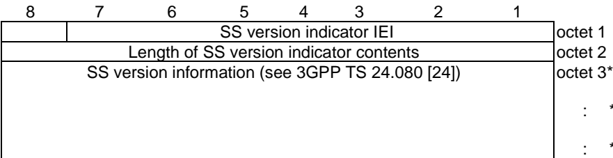
Figure 10.5.113/3GPP TS 24.008
