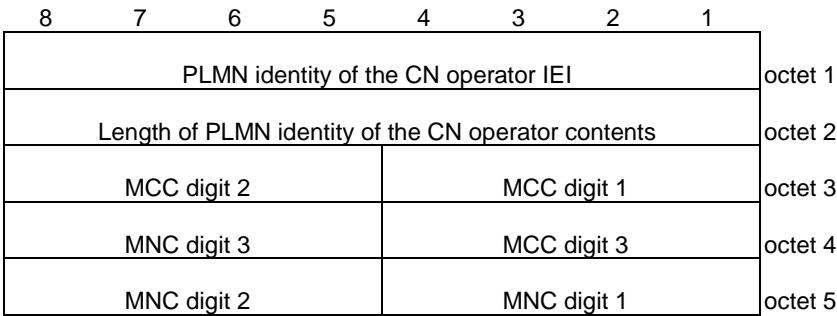
Figure 10.5.5.36-1/3GPP TS 24.008 PLMN identity of the CN operator information element
