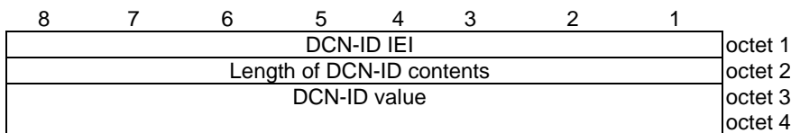
Figure 10.5.5.35-1/3GPP TS 24.008: DCN-ID information element
