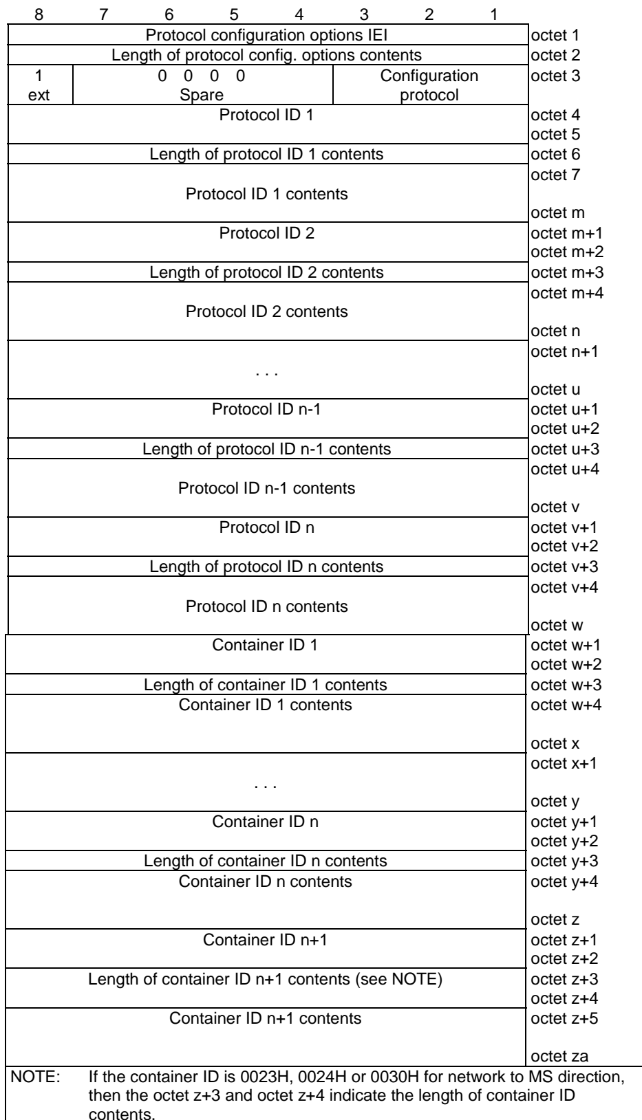
Figure 10.5.136/3GPP TS 24.008: Protocol configuration options information element
