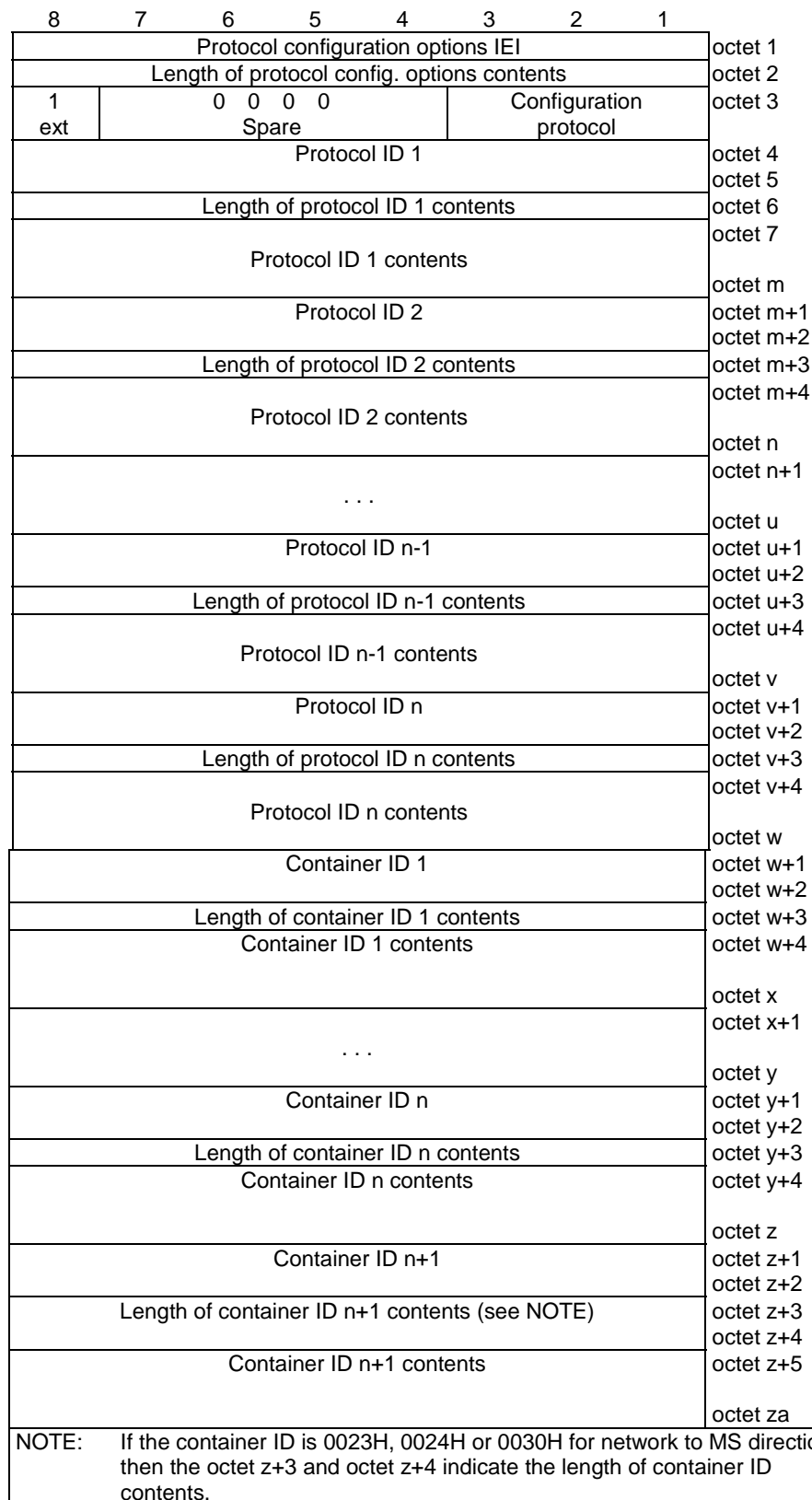
Figure 10.5.136/3GPP TS 24.008: Protocol configuration options information element
