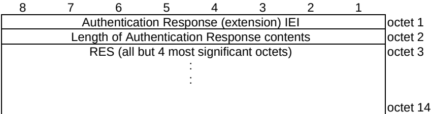
Figure 10.5.76.1/3GPP TS 24.008 Authentication Response Parameter (extension) information element (UMTS authentication challenge only)
