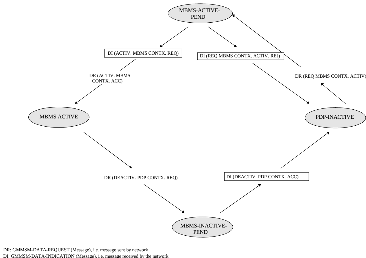
Figure 6.2a/3GPP TS 24.008: Session management states for MBMS context handling on the network side (overview)
