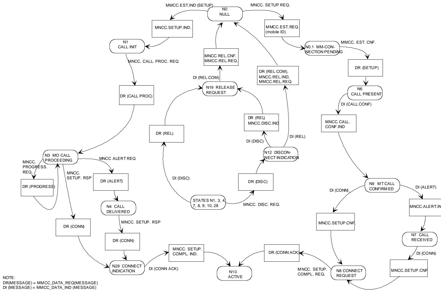
Figure 5.1b/3GPP TS 24.008 Overview call control protocol/Network side
