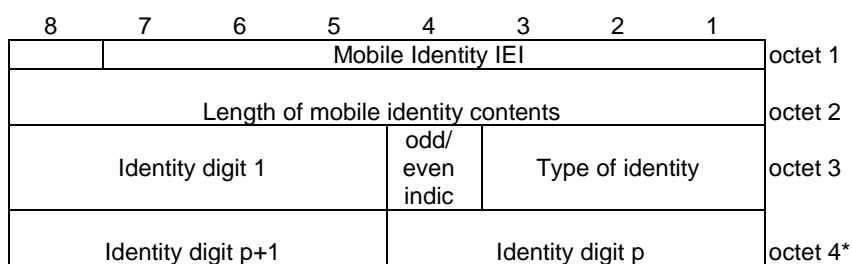
Figure 10.5.4/3GPP TS 24.008 Mobile Identity information element
