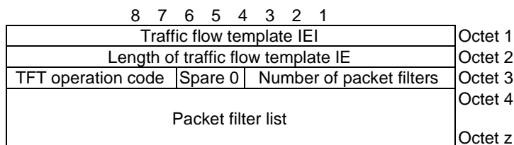
Figure 10.5.144/3GPP TS 24.008: Traffic flow template information element
