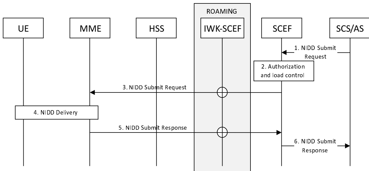
Figure 5.13.3-1: Mobile Terminated NIDD procedure
