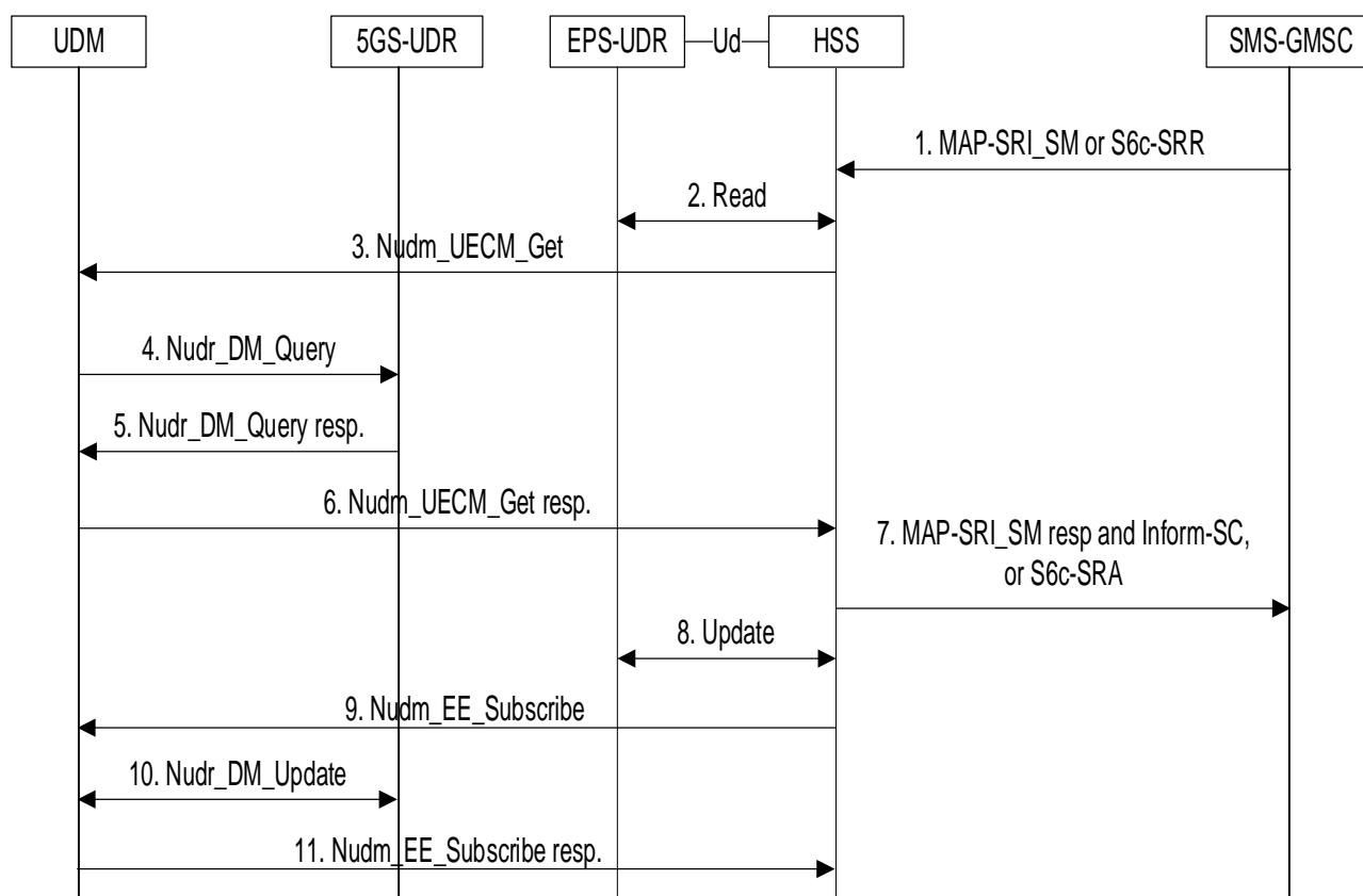
Figure 5.5.2-1: SMS Routing Info Retrieval
