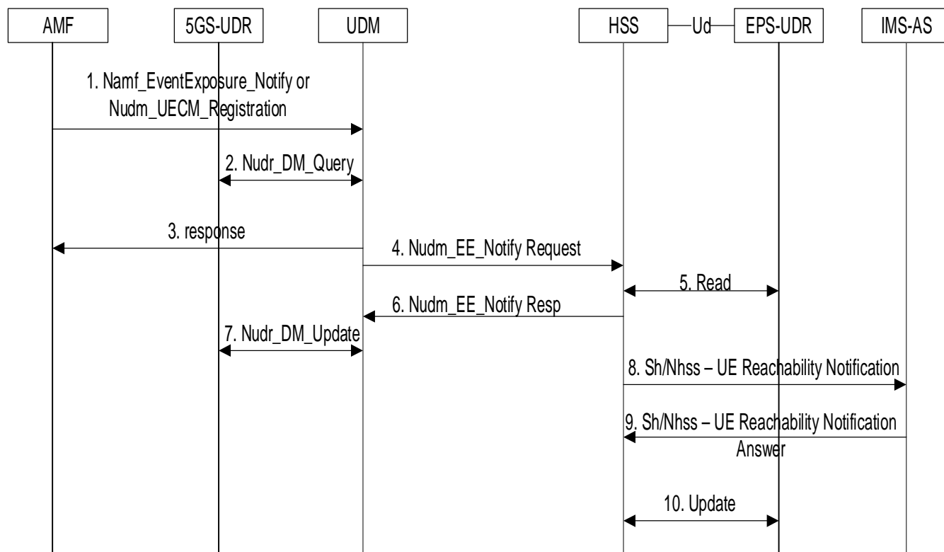
Figure 5.4.5-2: UE reachability notification for 5G subscriber
