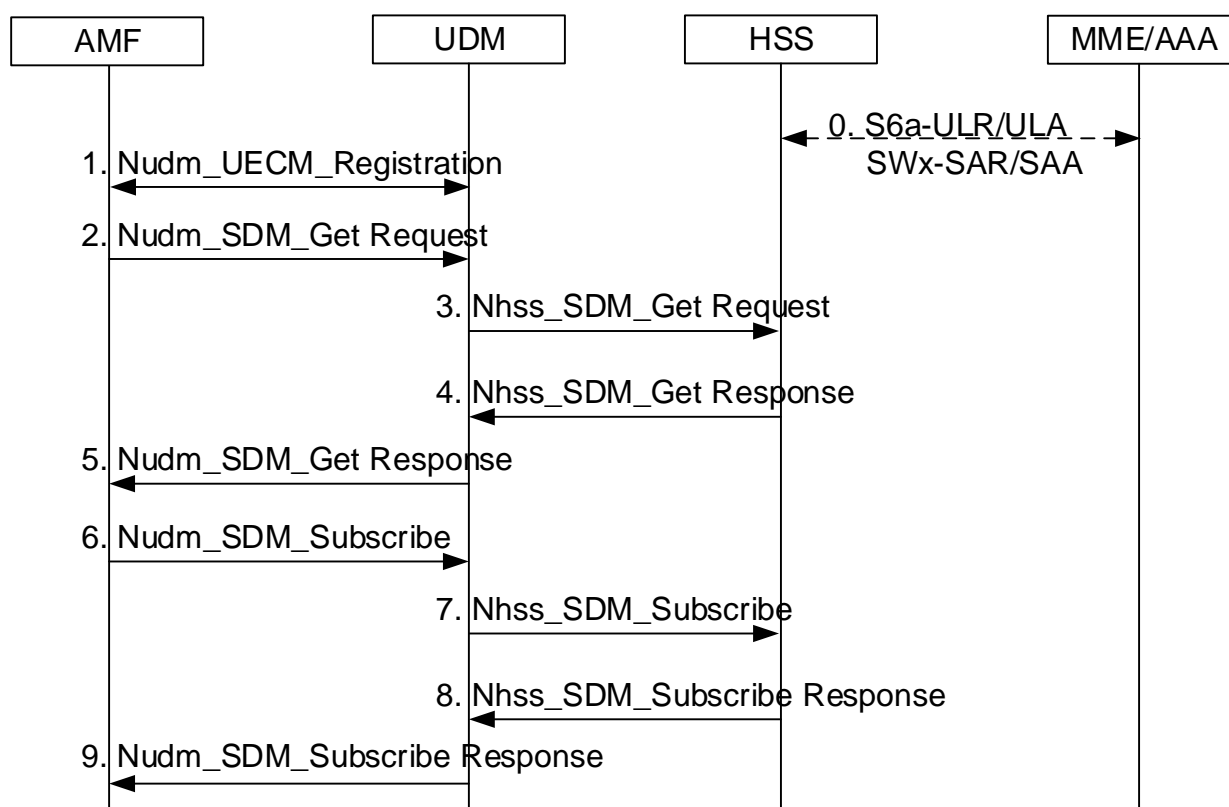
Figure 5.3.4-4: PDU session continuity during mobility from EPC/ePDG to 5GC
