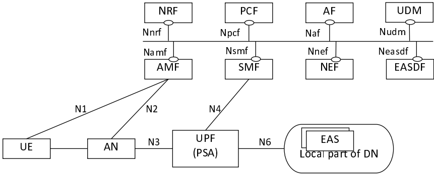
Figure 4.2-2: 5GS providing access to EAS without UL CL/BP for non-roaming scenario
