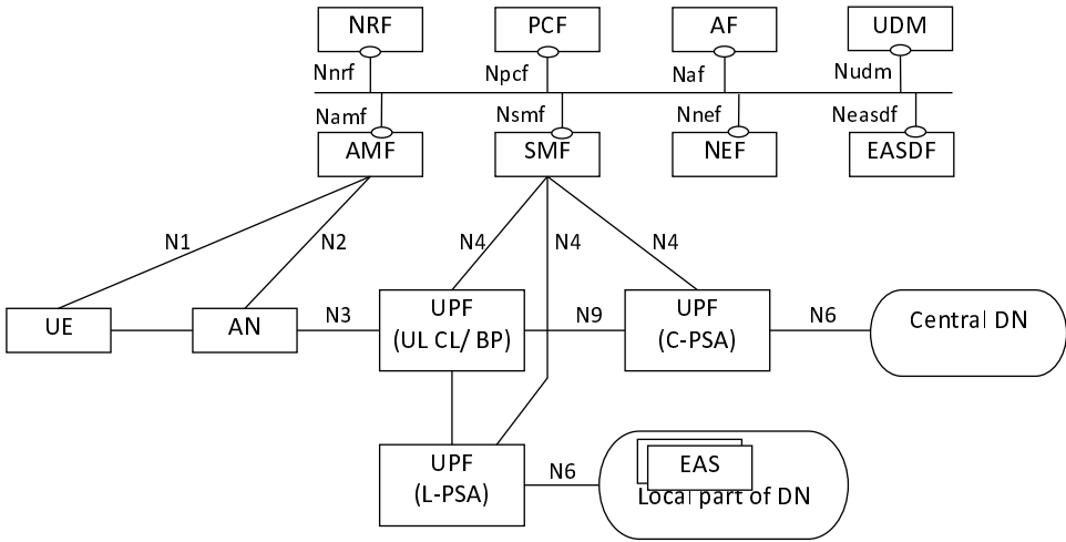
Figure 4.2-1: 5GS providing access to EAS with UL CL/BP for non-roaming scenario
