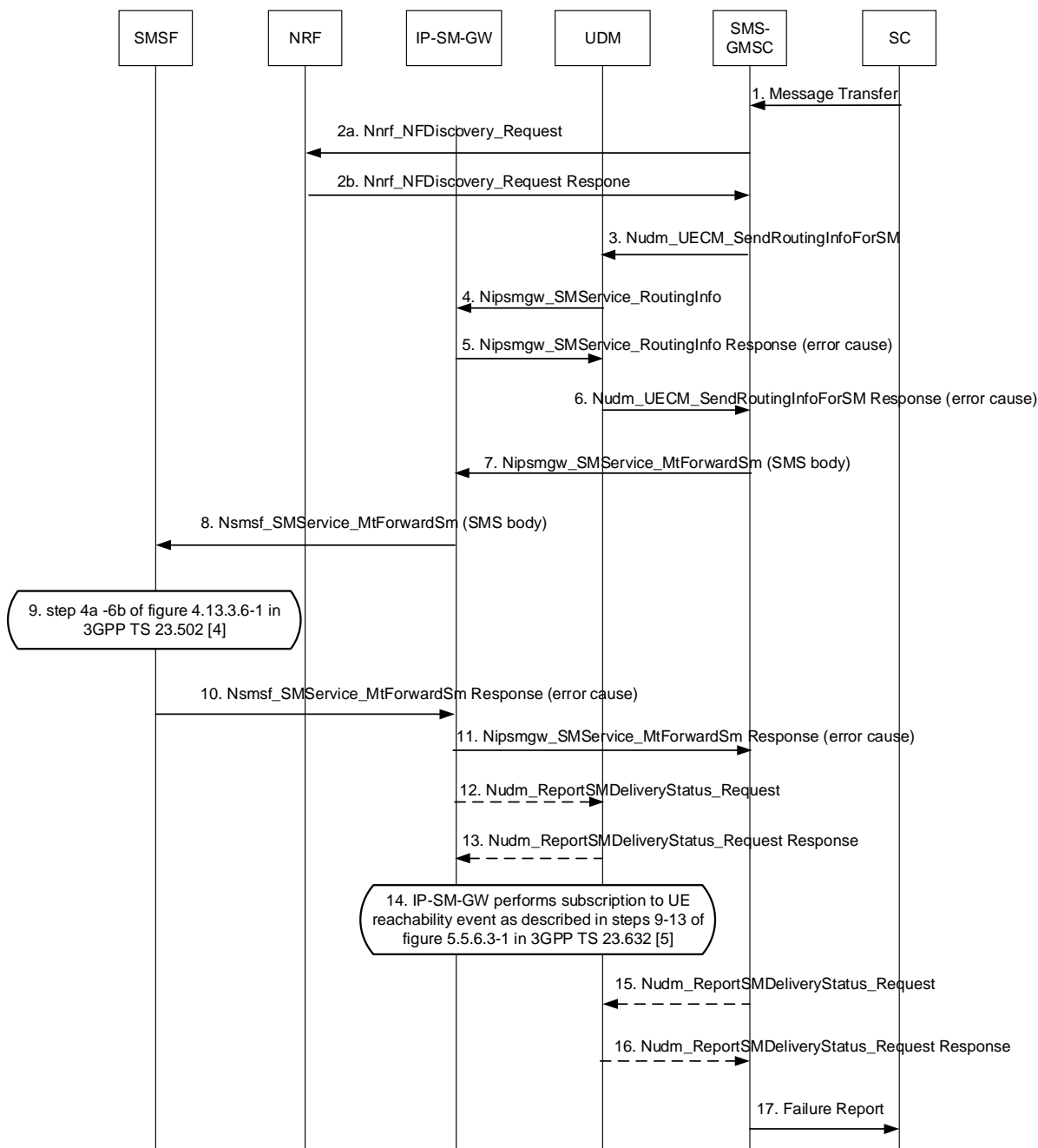
Figure 5.1.6-1: Unsuccessful MT SMS over NAS via IP-SM-GW
