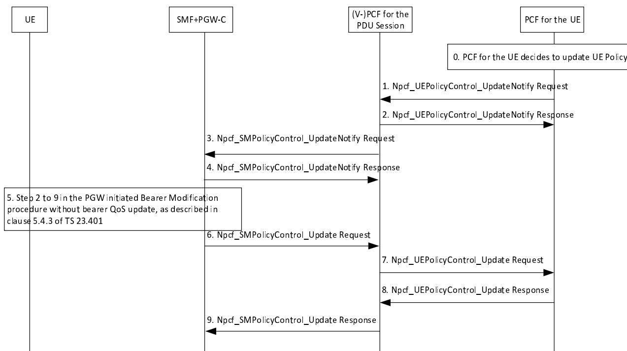
Figure 4.11.0a.2a.10-1: UE Policy Container delivery via EPS procedure
