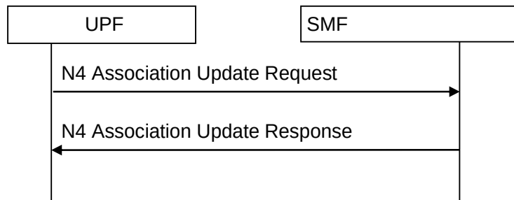
Figure 4.4.3.2-2: UPF initiated N4 association update procedure
