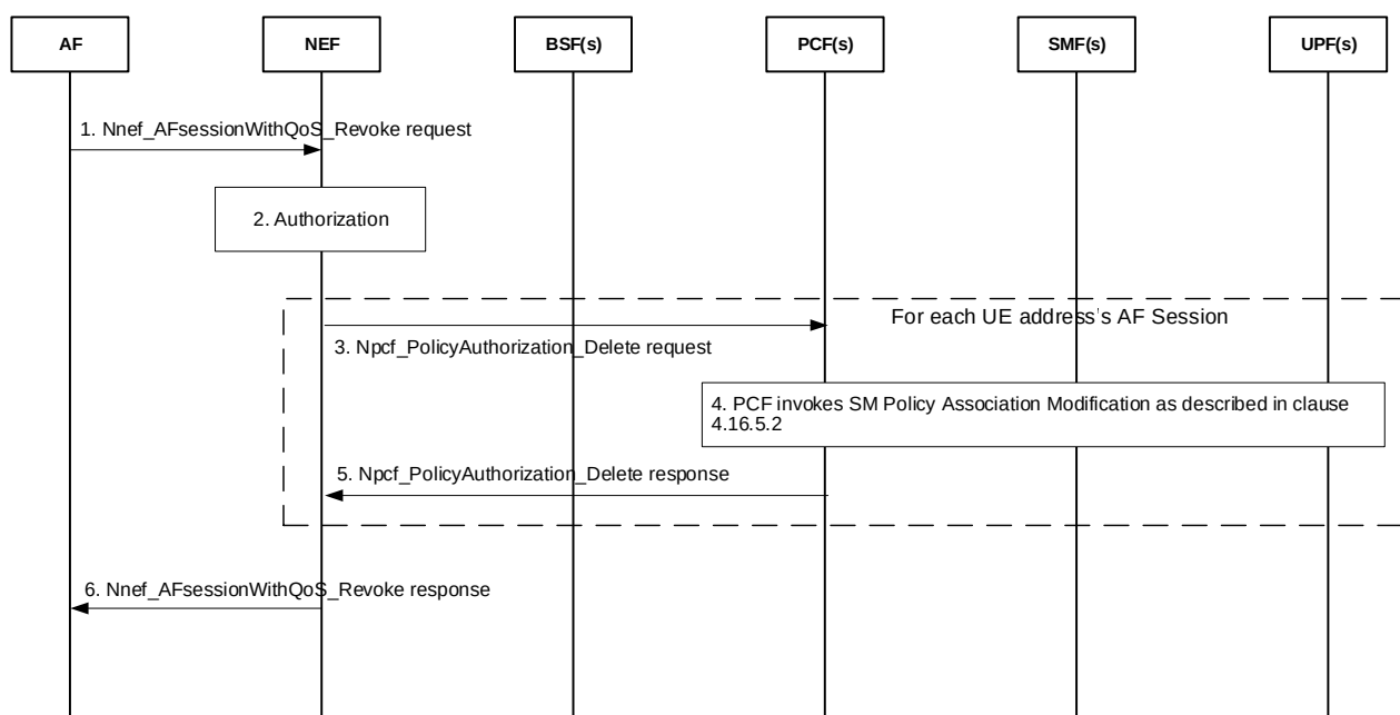
Figure 4.15.6.13.4-1: Procedure for revoking a Multi-member AF session with required QoS
