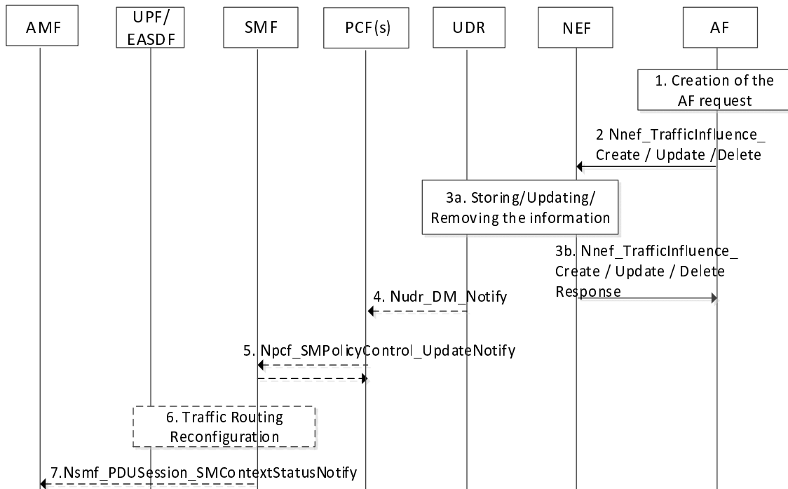
Figure 4.3.6.2-1: Processing AF requests to influence traffic routing for Sessions not identified by an UE address
