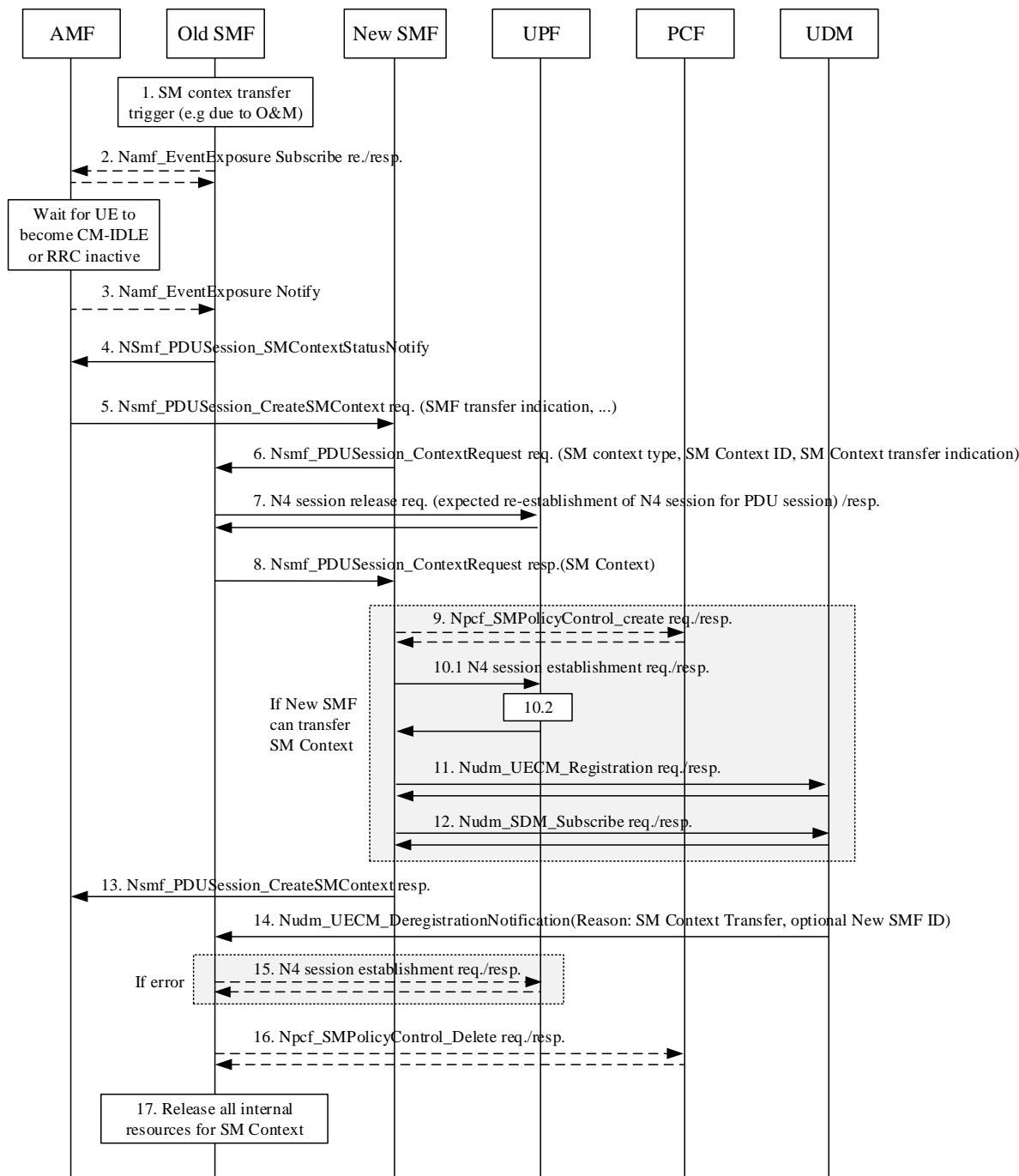
Figure 4.26.4.1.1-1: Context transfer of a PDU session
