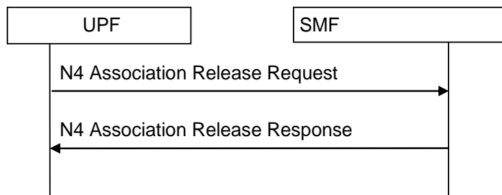
Figure 4.4.3.3-2: UPF initiated N4 association release procedure
