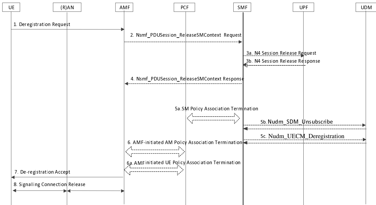
Figure 4.2.2.3.2-1: UE-initiated Deregistration
