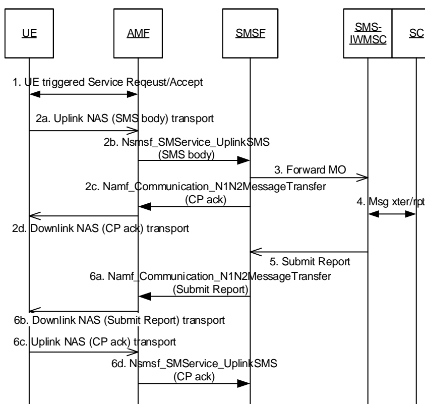
Figure 4.13.3.3-1: MO SMS over NAS
