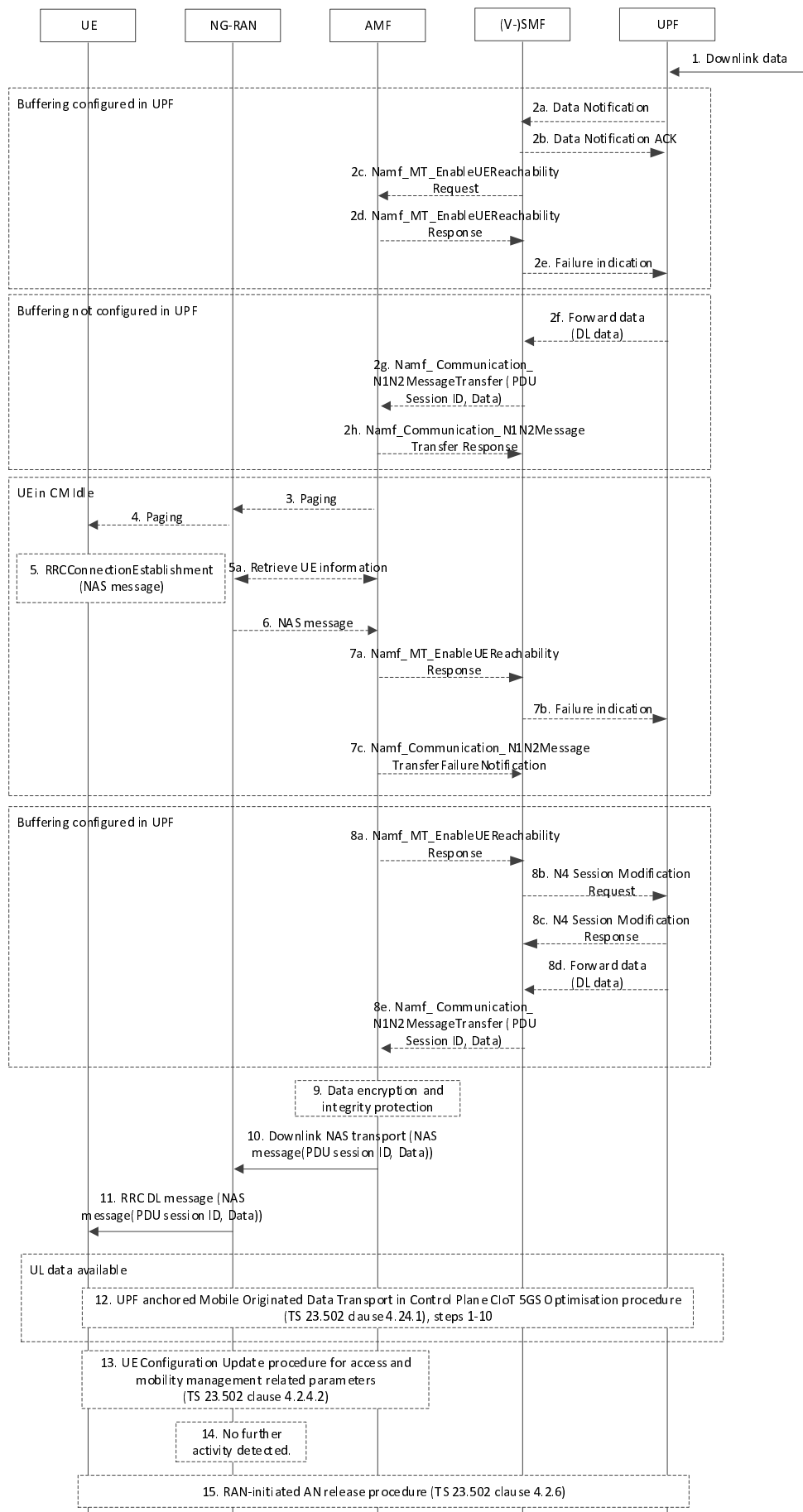
Figure 4.24.2-1: Mobile Terminated Data Transport in Control Plane IoT 5GS Optimisation
