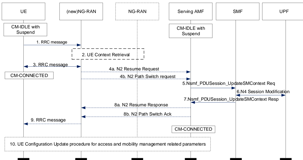
Figure 4.8.2.3-1: Connection Resume in CM-IDLE with Suspend
