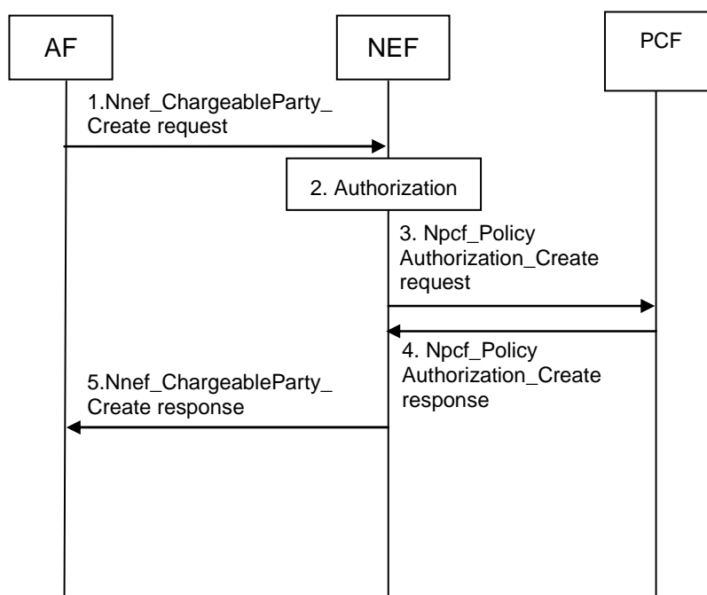
Figure 4.15.6.4-1: Set the chargeable party at AF session set-up
