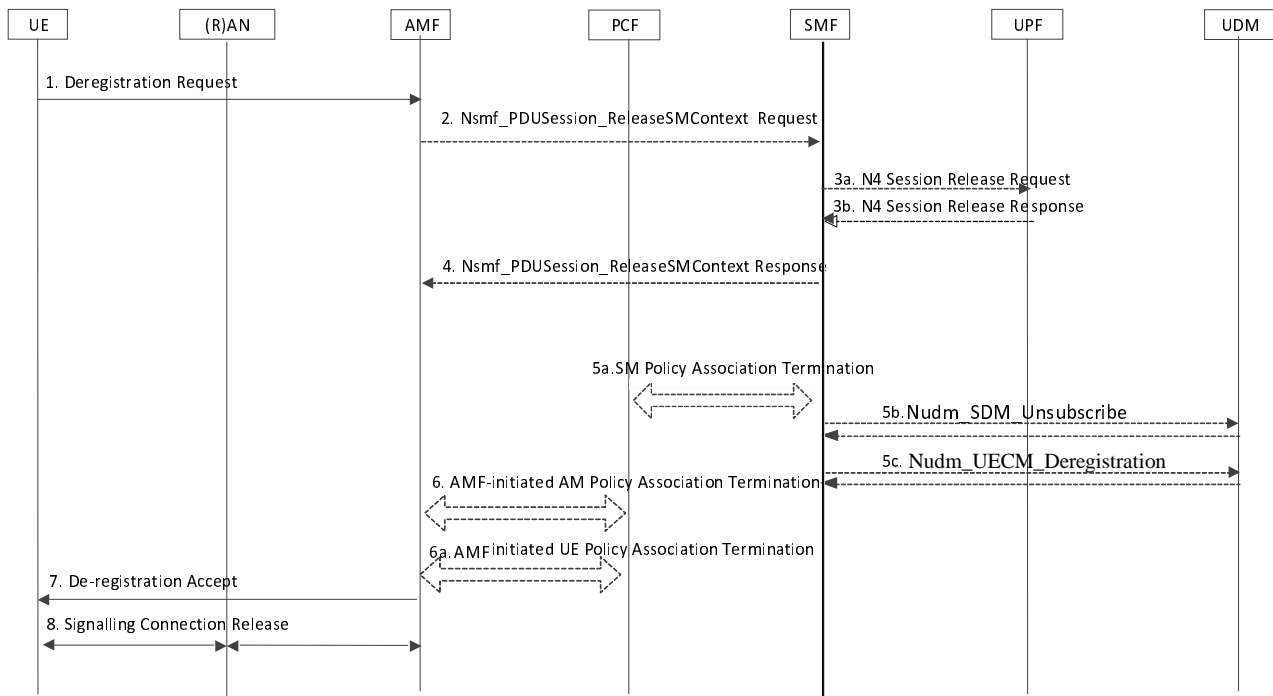
Figure 4.2.2.3.2-1: UE-initiated Deregistration
