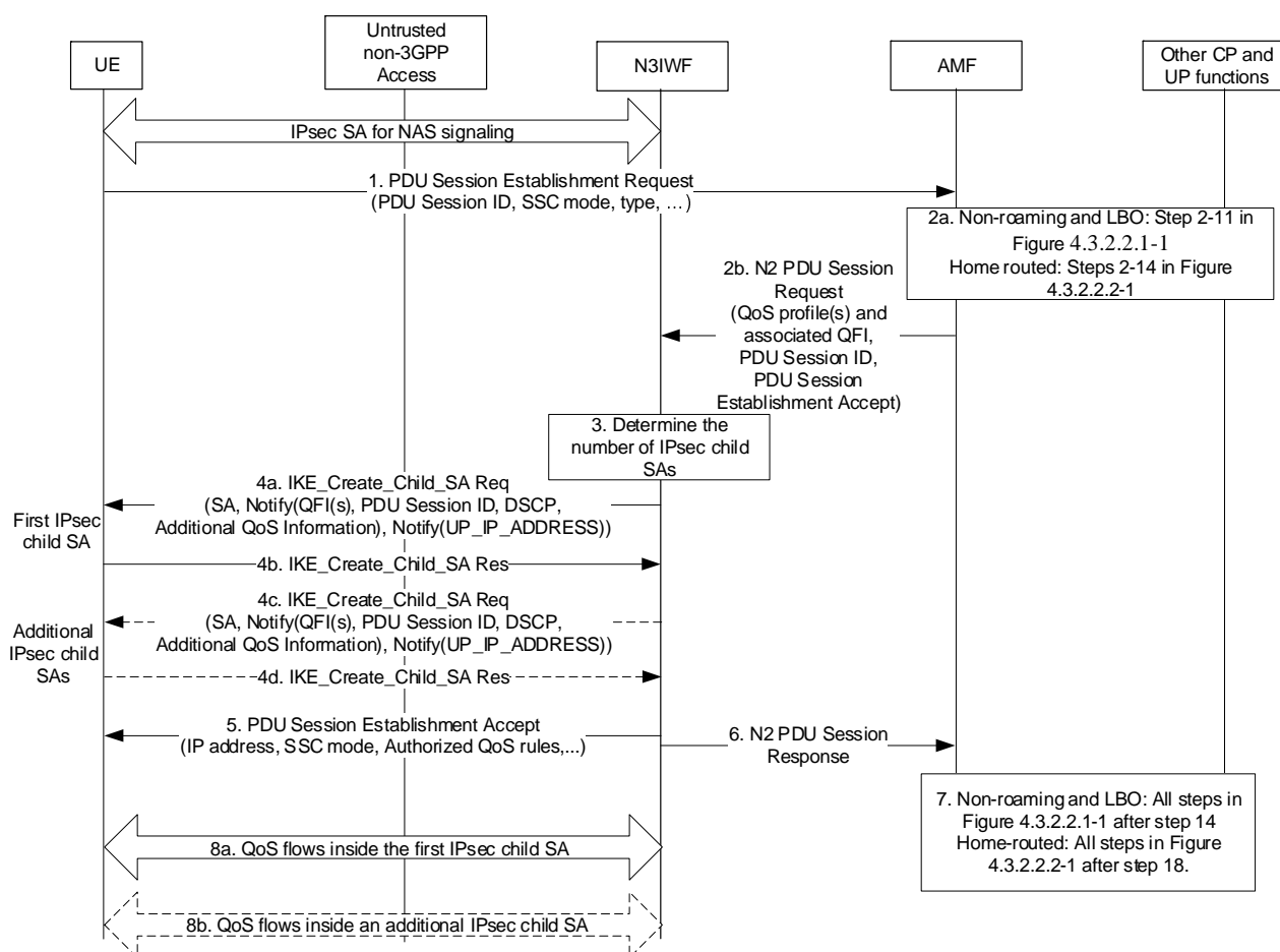
Figure 4.12.5-1: PDU Session establishment via untrusted non-3GPP access
