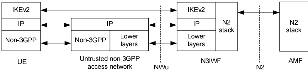
Figure 8.2.4-3: Control Plane for establishment of user-plane via N3IWF
