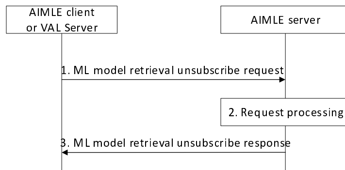
Figure 8.2.2.3.5-1: ML model retrieval unsubscribe
