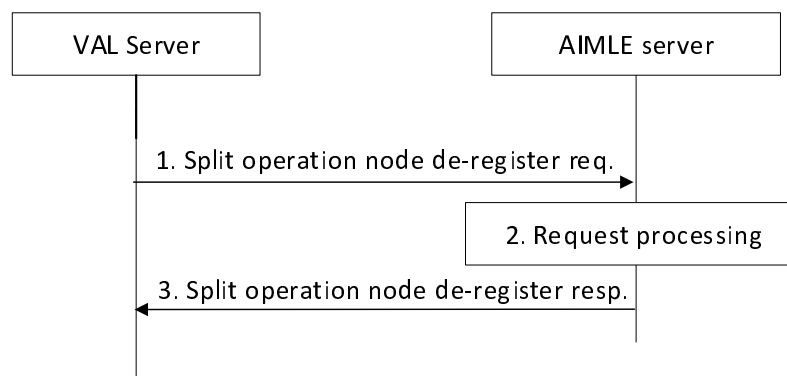
Figure 8.14.2.4.4-1: Split operation node de-registration
