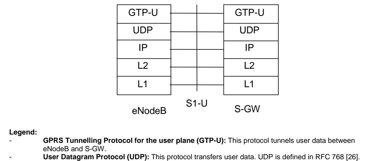
Figure 5.1.2.2-1: User Plane for eNodeB – S-GW
