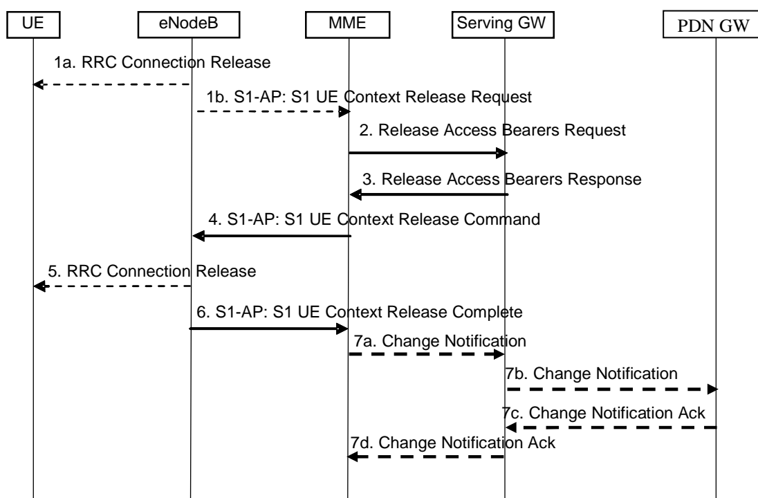
Figure 5.3.5-1: S1 Release Procedure
