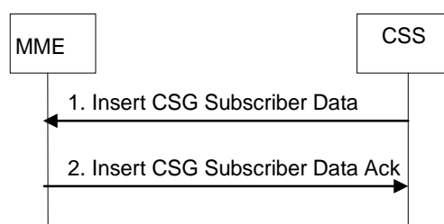
Figure 5.3.13.2-1: Insert CSG Subscriber Data procedure
