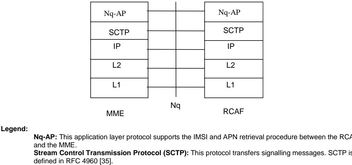
Figure 5.1.1.13-1: Control Plane for Nq interface
