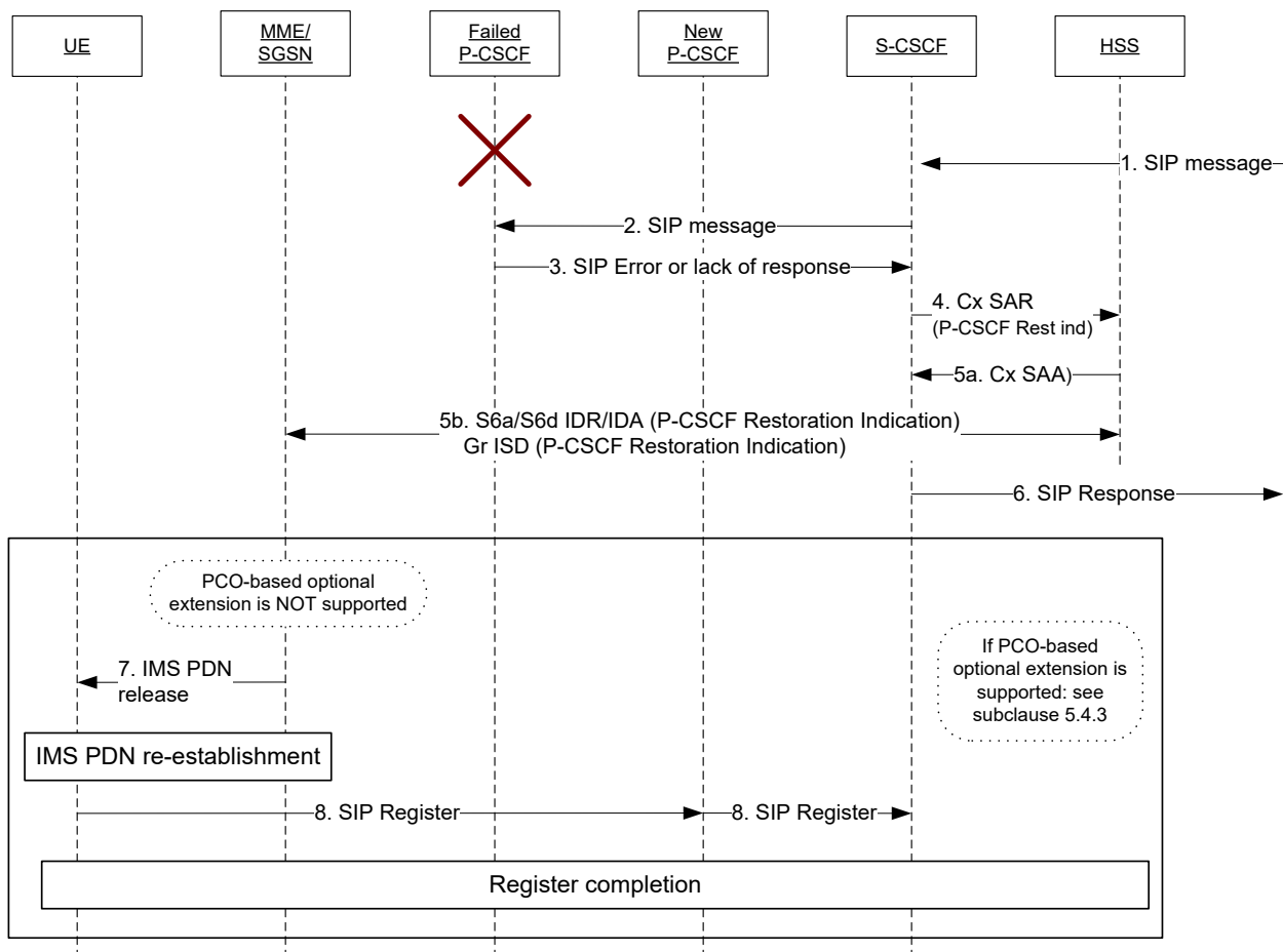
Figure 5.4.2.1-1: HSS-based P-CSCF restoration
