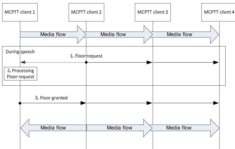
Figure 10.9.2.7-1: Floor request with override authorization
