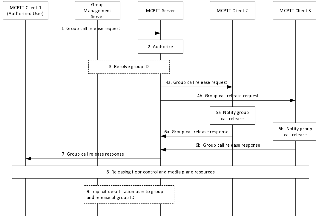
Figure 10.6.2.8.3-1: Group call end (by authorized user) for temporary group call – user regroup
