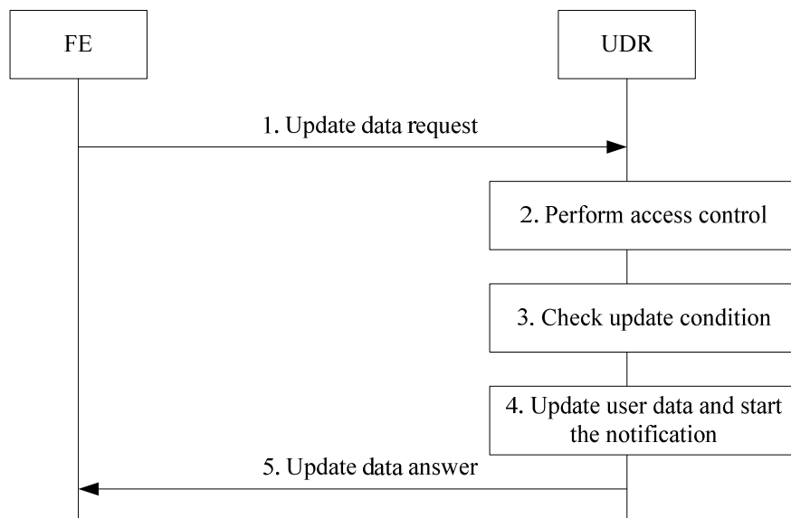
Figure 5.6-1: Update data procedure
