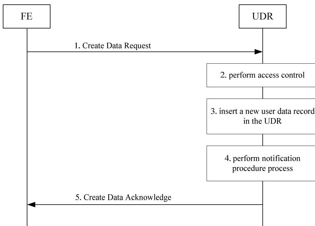
Figure 5.4-1 Create Data flow
