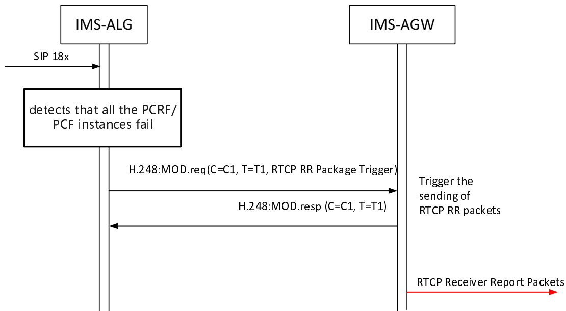
Figure 6.2.26.1: Procedure to triggering RTCP RR packets
