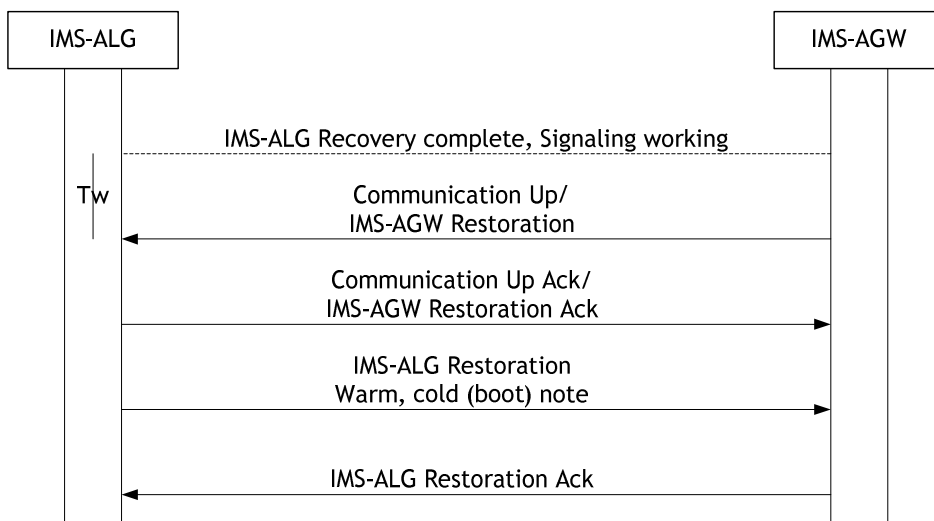
Figure 6.1.5.2.1: IMS-ALG Restoration
