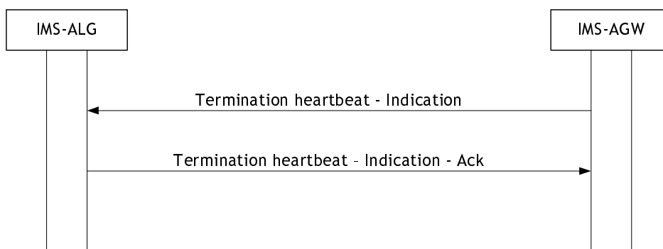
Figure 6.2.6.1: Termination heartbeat – Indication
