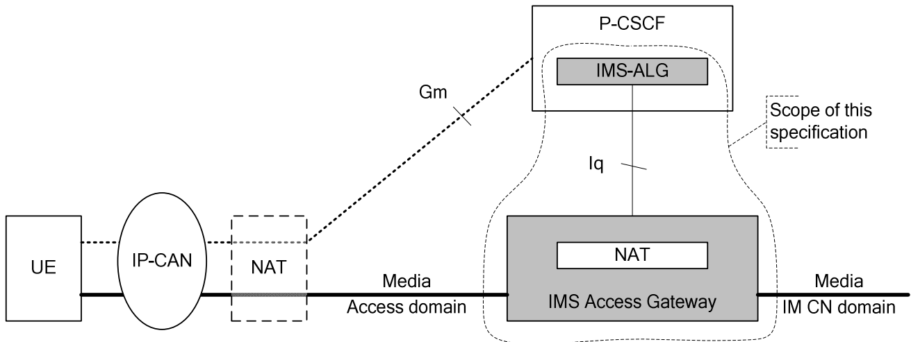
Figure 1.1: Scope of the specification
