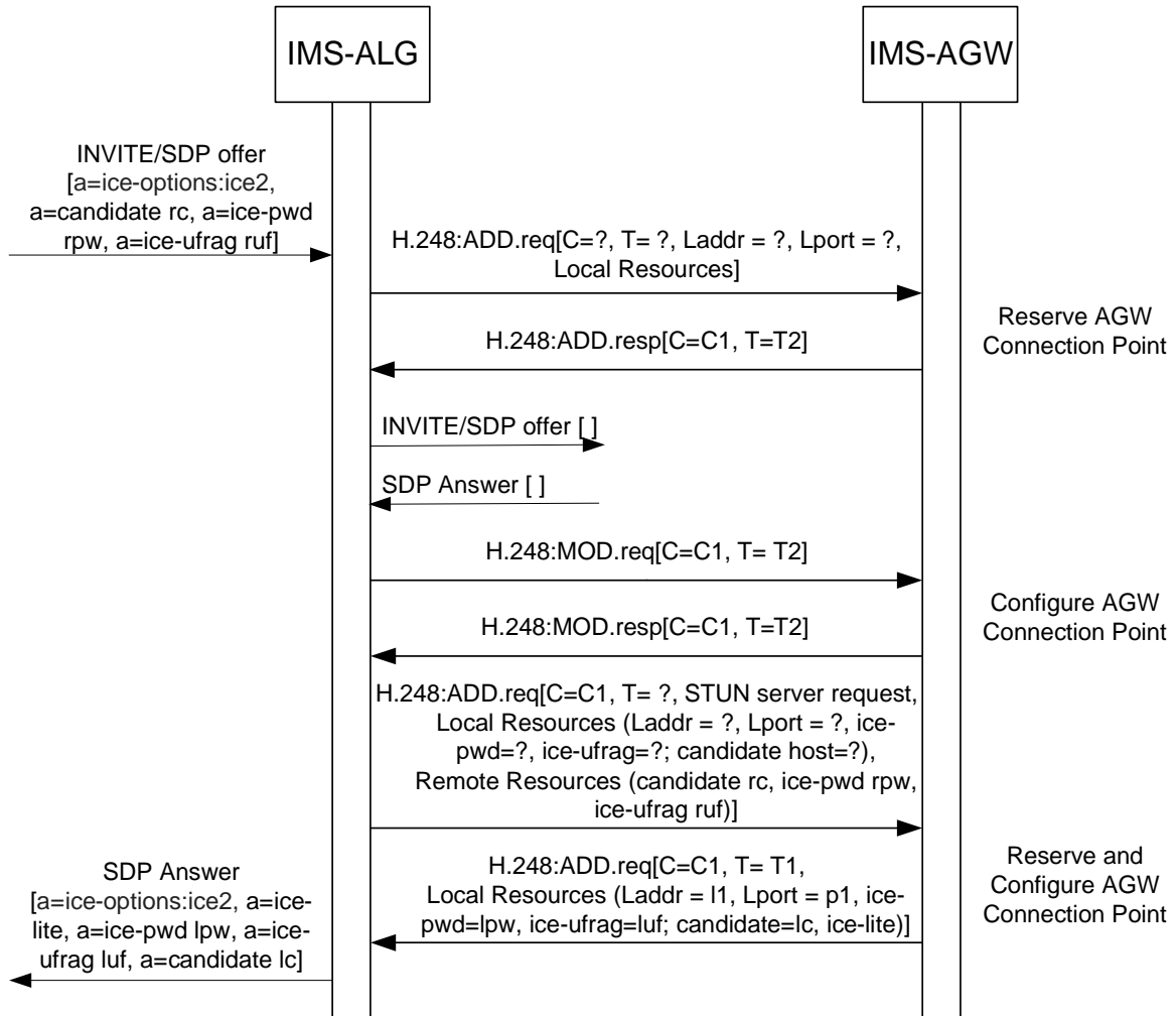
Figure 6.2.17.1.1: Procedure for interactive connectivity establishment using ICE lite towards the offerer
