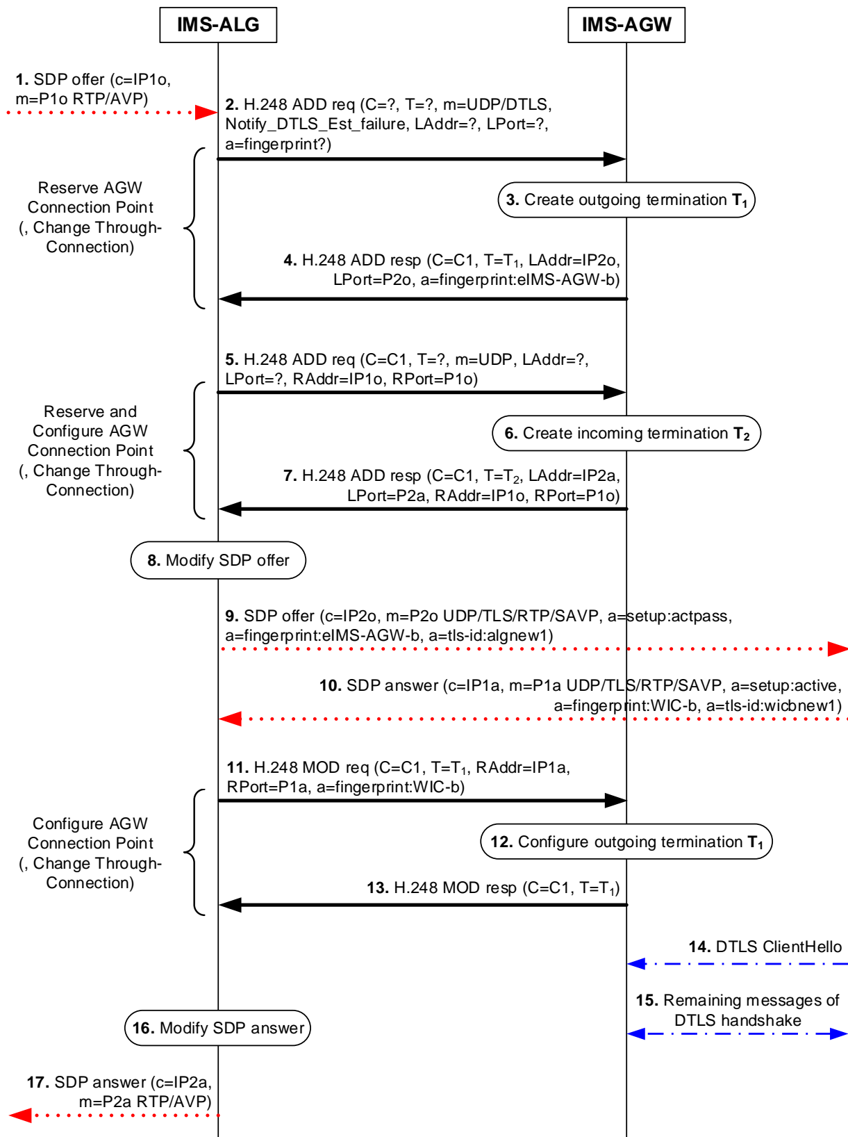
Figure 6.2.10.5.2: UE terminated procedure using DTLS-SRTP
