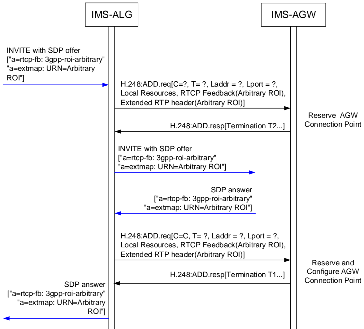
Figure 6.2.21.3.1: Procedure to indicate Arbitrary ROI mode
