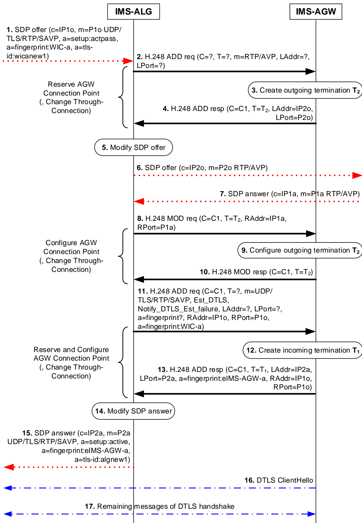
Figure 6.2.10.5.1: UE originated procedure using DTLS-SRTP
