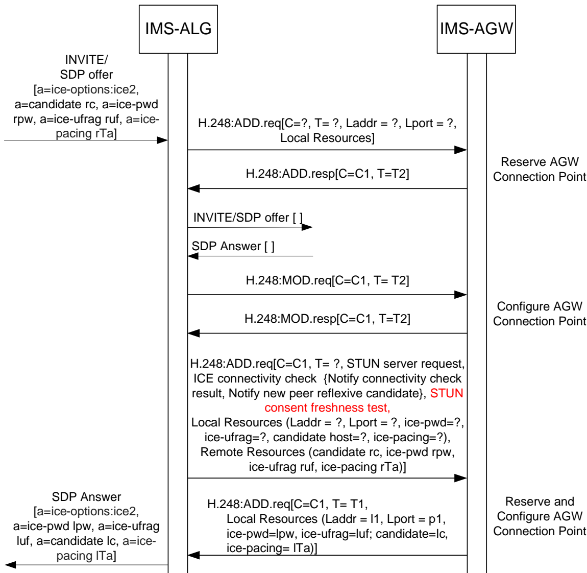
Figure 6.2.17.5.1: Procedure for STUN consent freshness test towards the offerer
