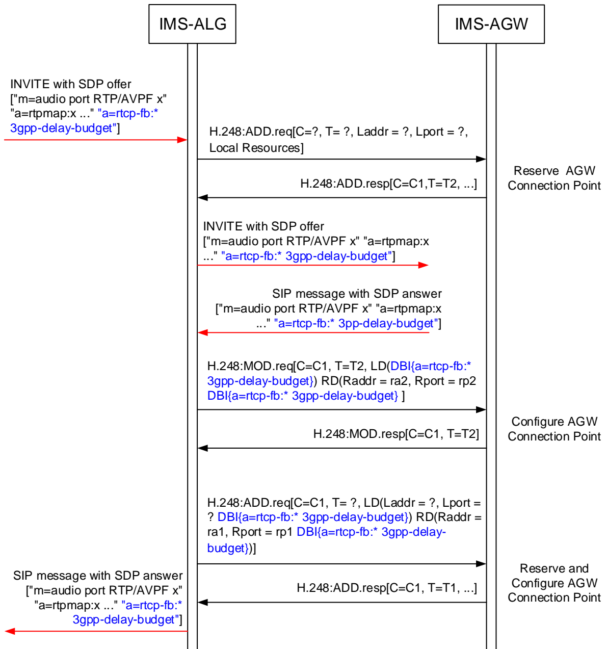
Figure 6.2.25.1: Procedure to indicate DBI
