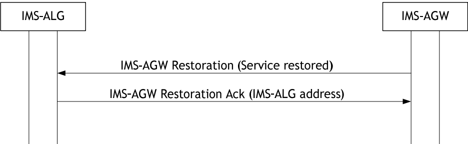
Figure 6.1.4.1: IMS-AGW Restoration
