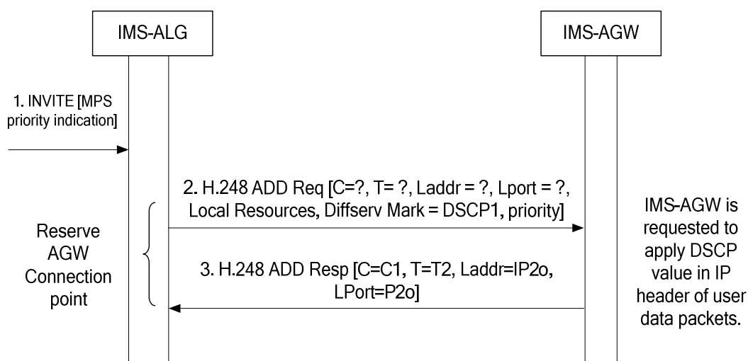
Figure 6.2.15.5.1: Request to reserve IMS-AGW call resources and apply DSCP marking for MPS
