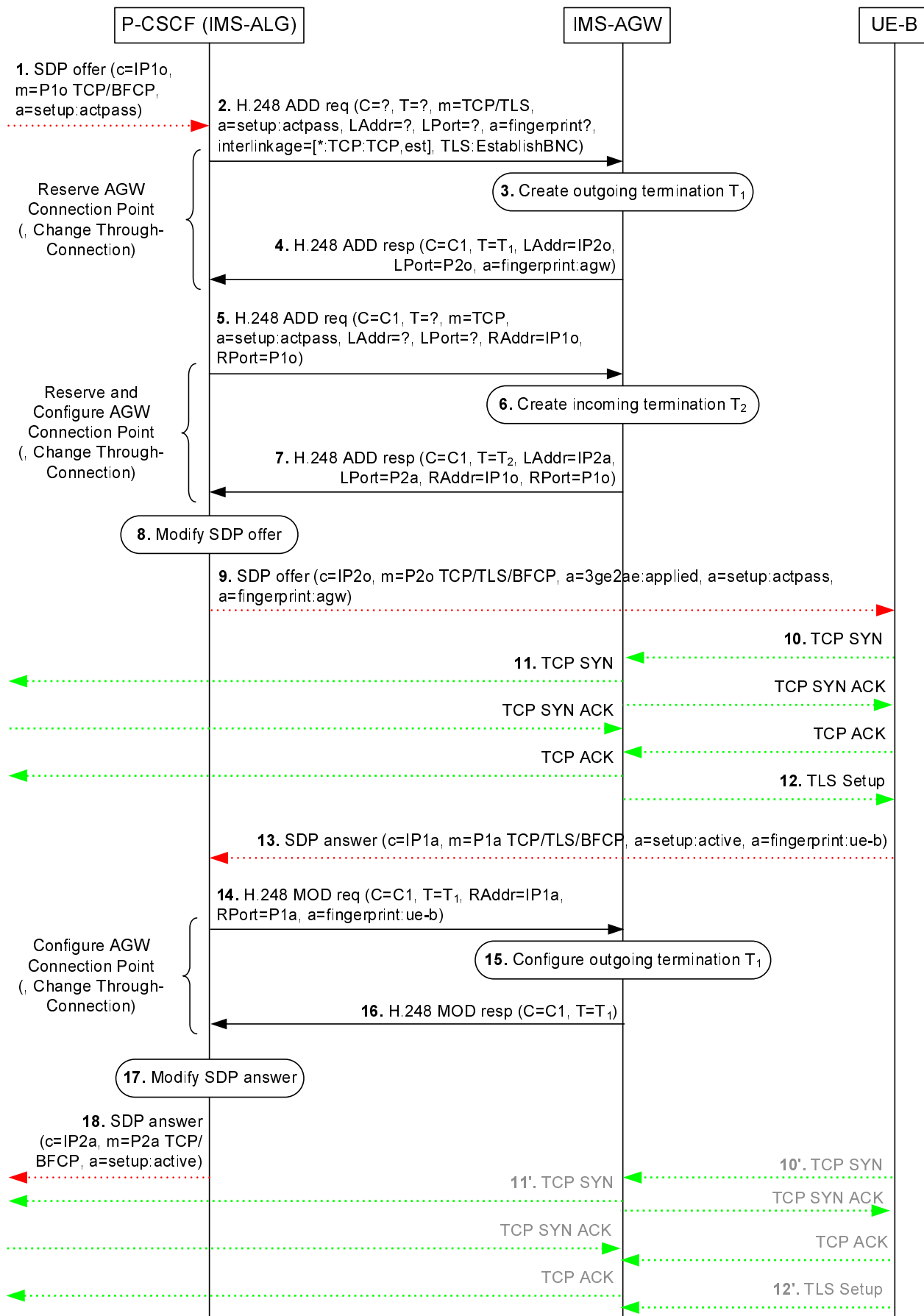
Figure 6.2.10.3.2.2.1.1: Terminating example call flow for e2e security for MSRP where an incoming TCP bearer establishment triggers an outgoing TCP bearer establishment
