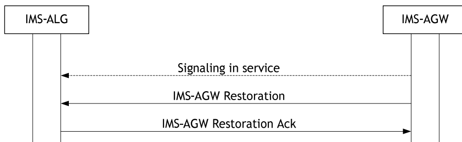
Figure 6.1.3.2: IMS-AGW indicates recovery from a failure/or maintenance unlocking
