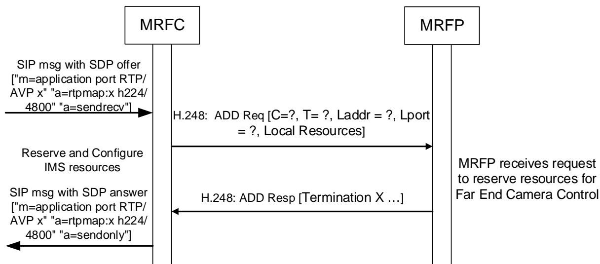
Figure 6.2.22.1.1: Procedure to indicate Video ROI using FECC
