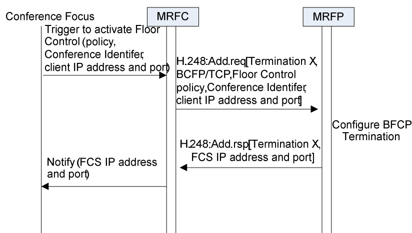
Figure 6.2.13.2.1: Configure Floor Control Termination
