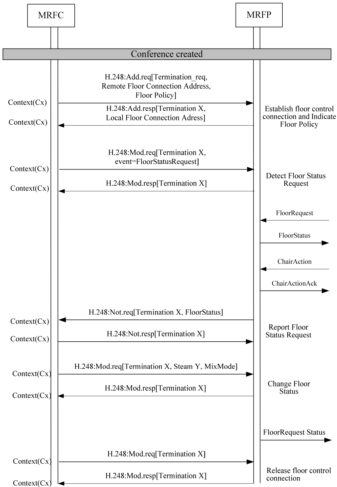
Figure 6.2.13.1 Floor control (message sequence chart)
