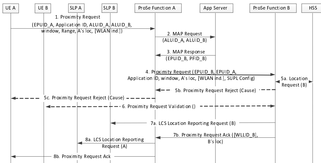
Figure 5.5.5-1: Proximity Request
