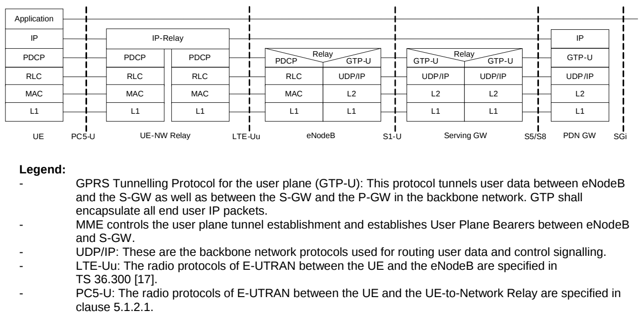
Figure 5.1.2.2-1: User Plane for UE-to-Network Relay
